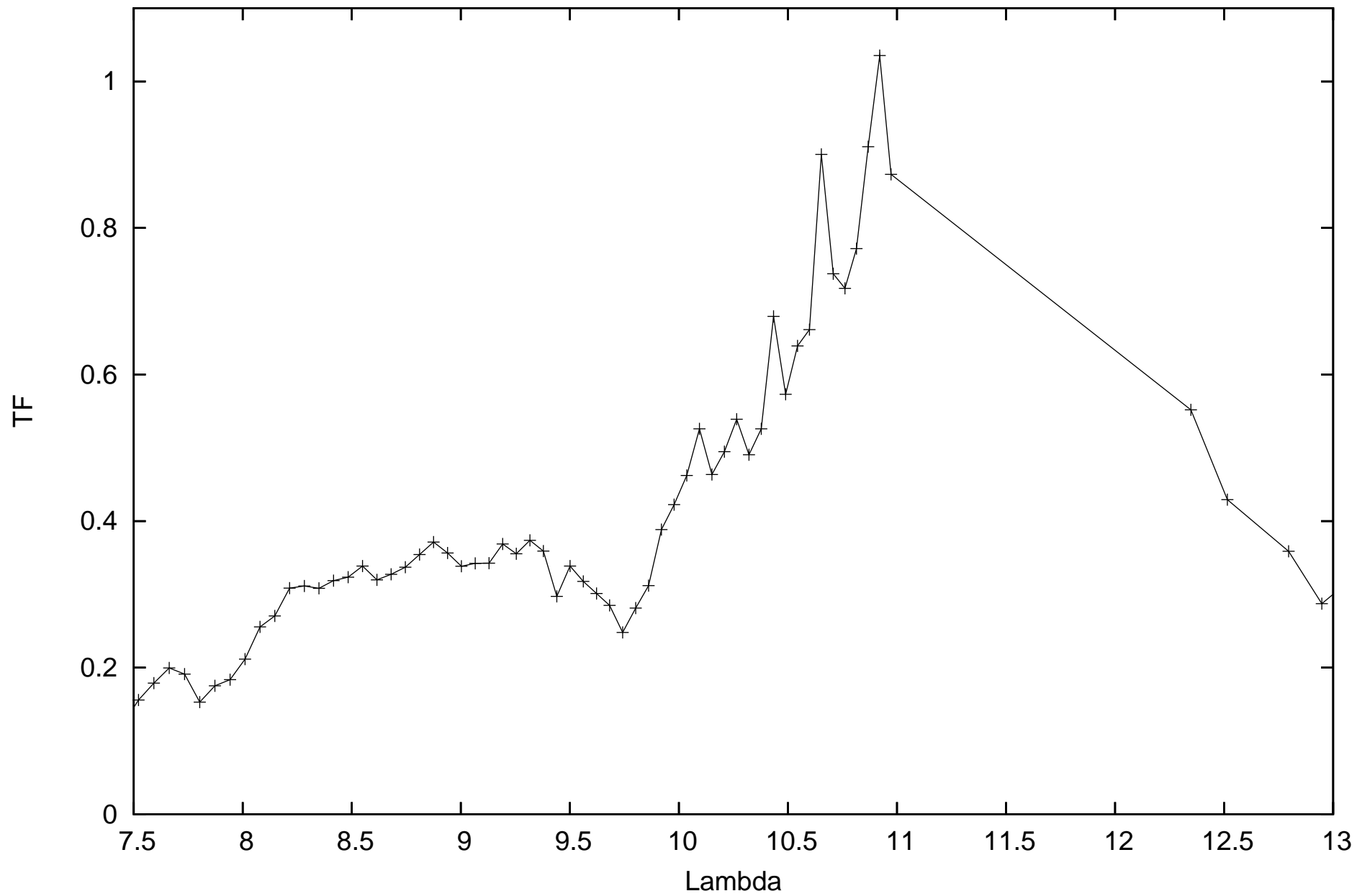
calHD202369_flux0.29_diam4.56_r.MIDI.2008-09-27T03_53_16.000_HIGHSENS
