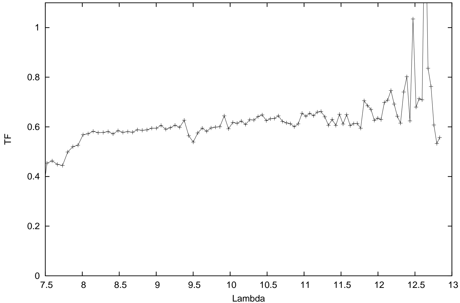
calHD169916_flux0.26_diam3.99_r.MIDI.2009-08-18T03_31_10.000_HIGHSENS
