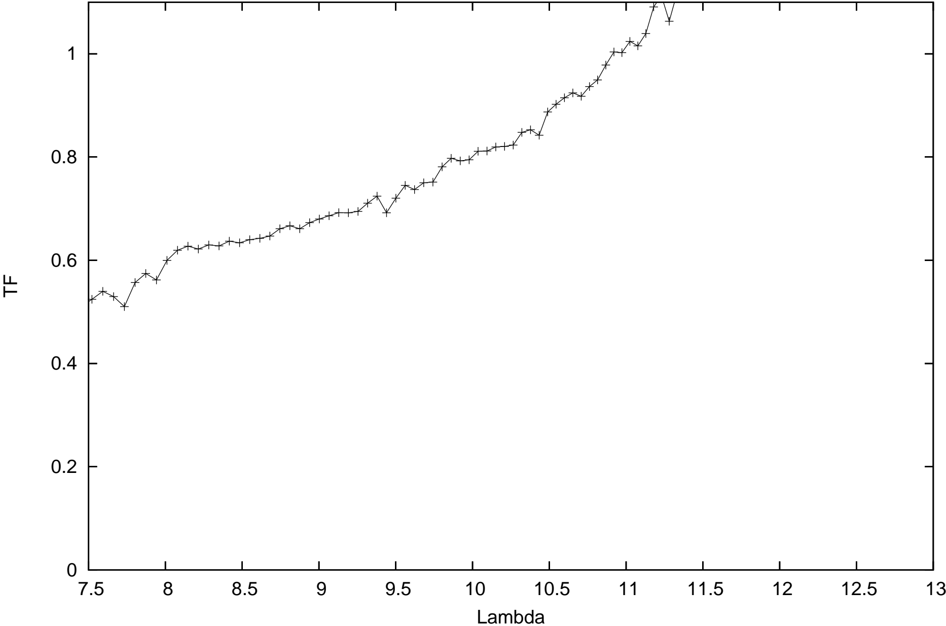
calHD168454_flux-0.48_diam5.87_r.MIDI.2009-07-05T04_46_22.000_HIGHSENS
