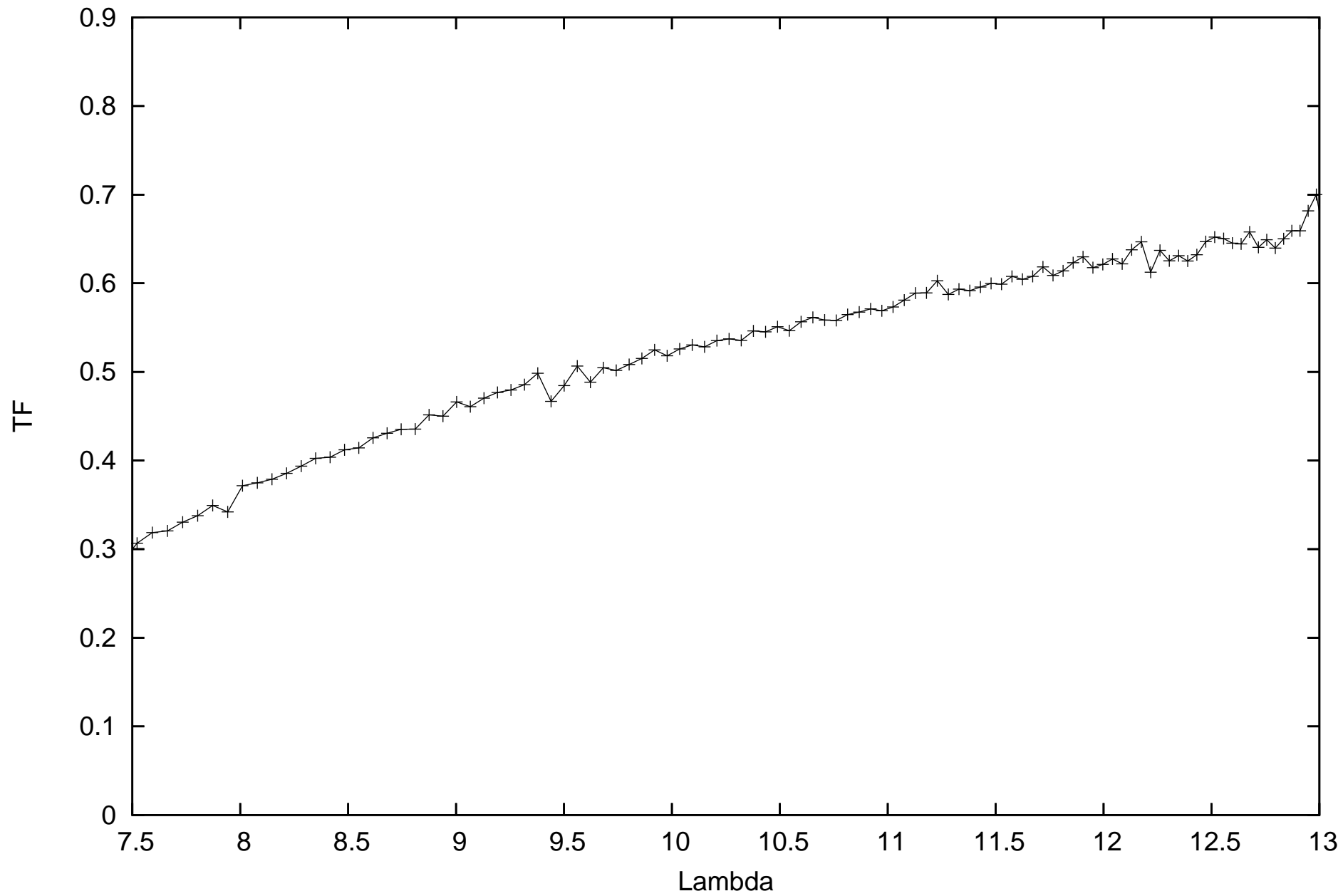
calHD167618_flux-1.82_diam11.66_r.MIDI.2009-10-20T01_57_48.000_G1H0
