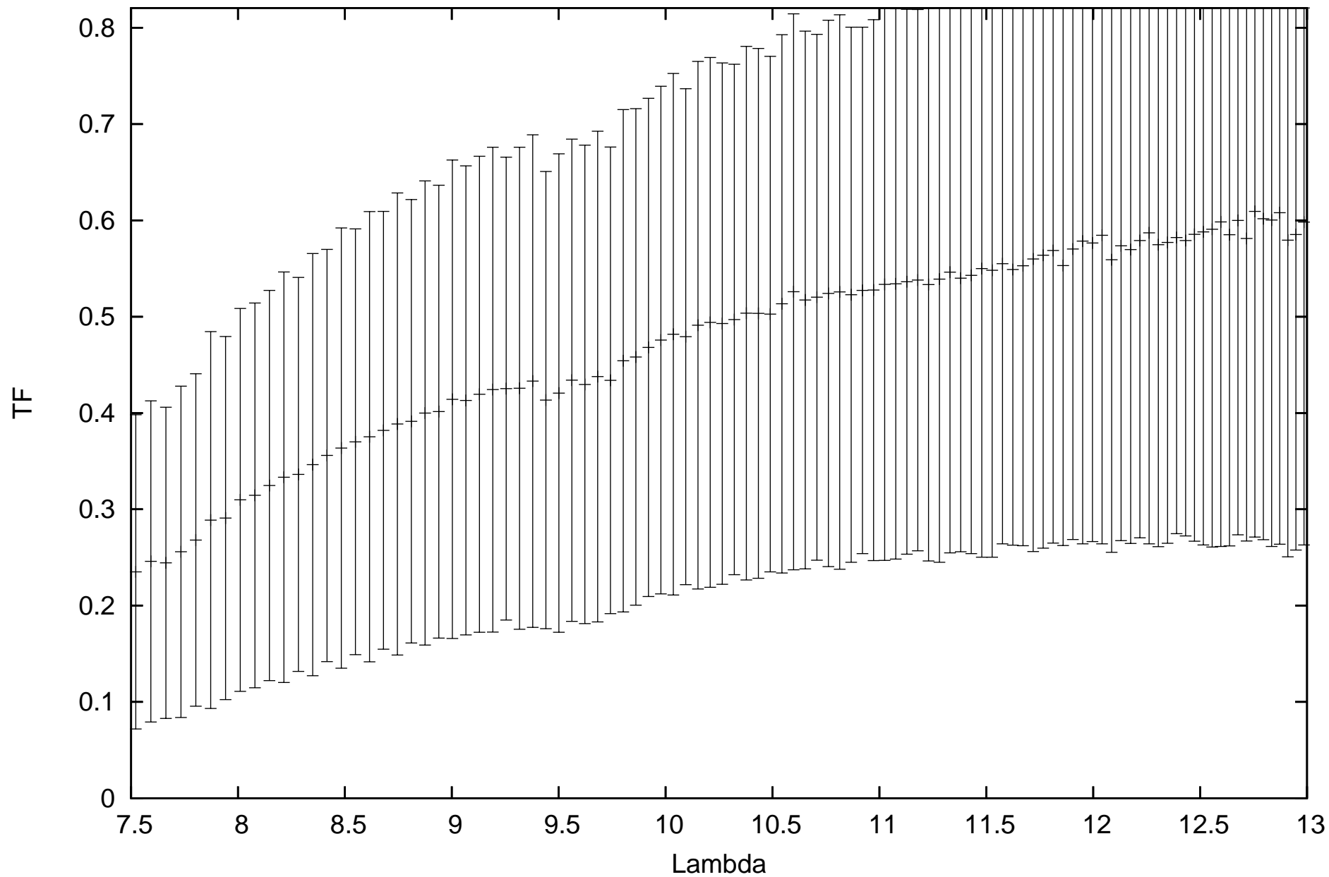
calHD167618_flux-1.82_diam11.66_r.MIDI.2009-09-27T00_23_33.000_HIGHSENS
