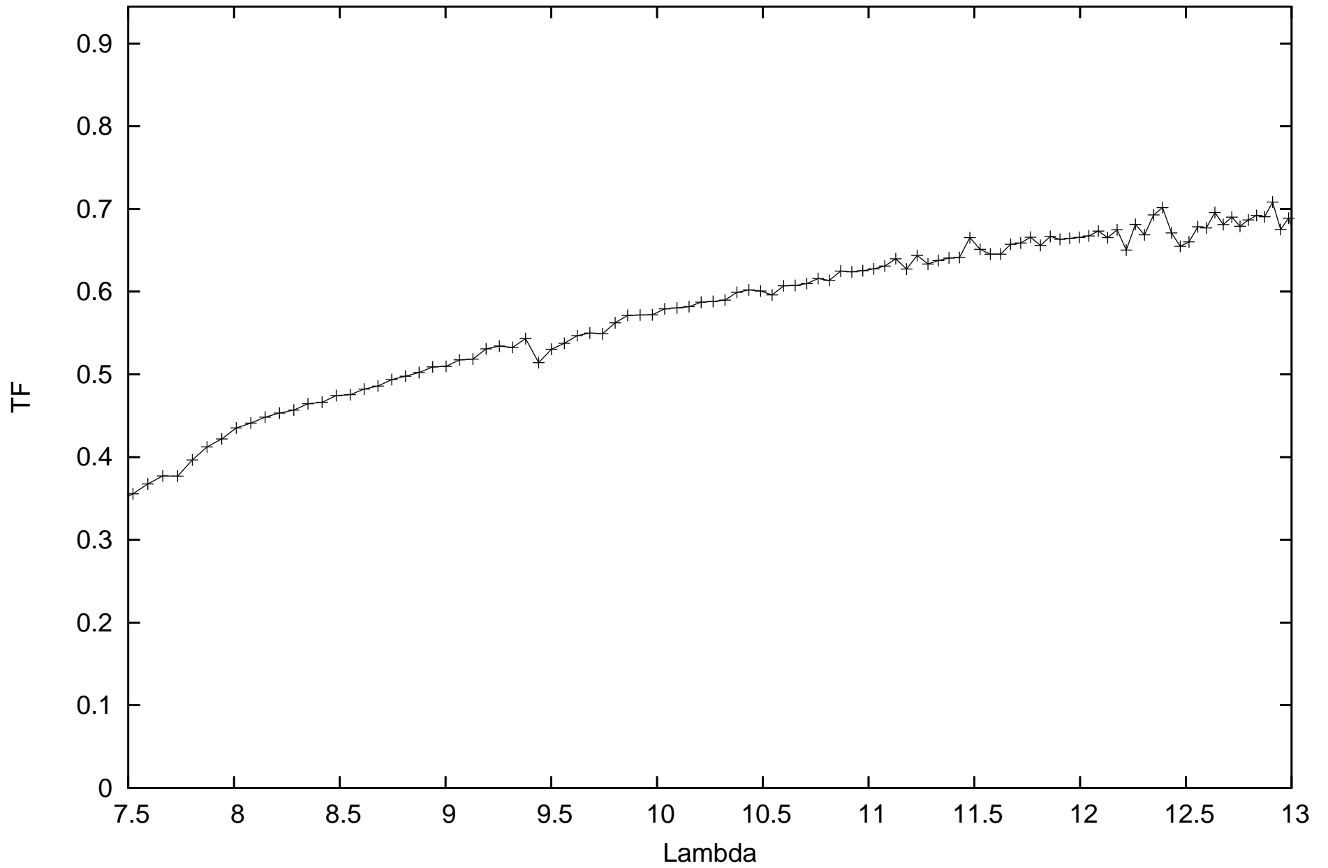
calHD167618_flux-1.82_diam11.66_r.MIDI.2009-09-26T23_45_09.000_HIGHSENS
