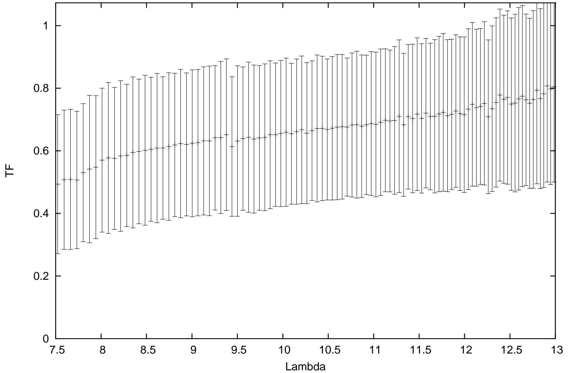
calHD167618_flux-1.82_diam11.66_r.MIDI.2009-08-18T03_06_05.000_HIGHSENS
