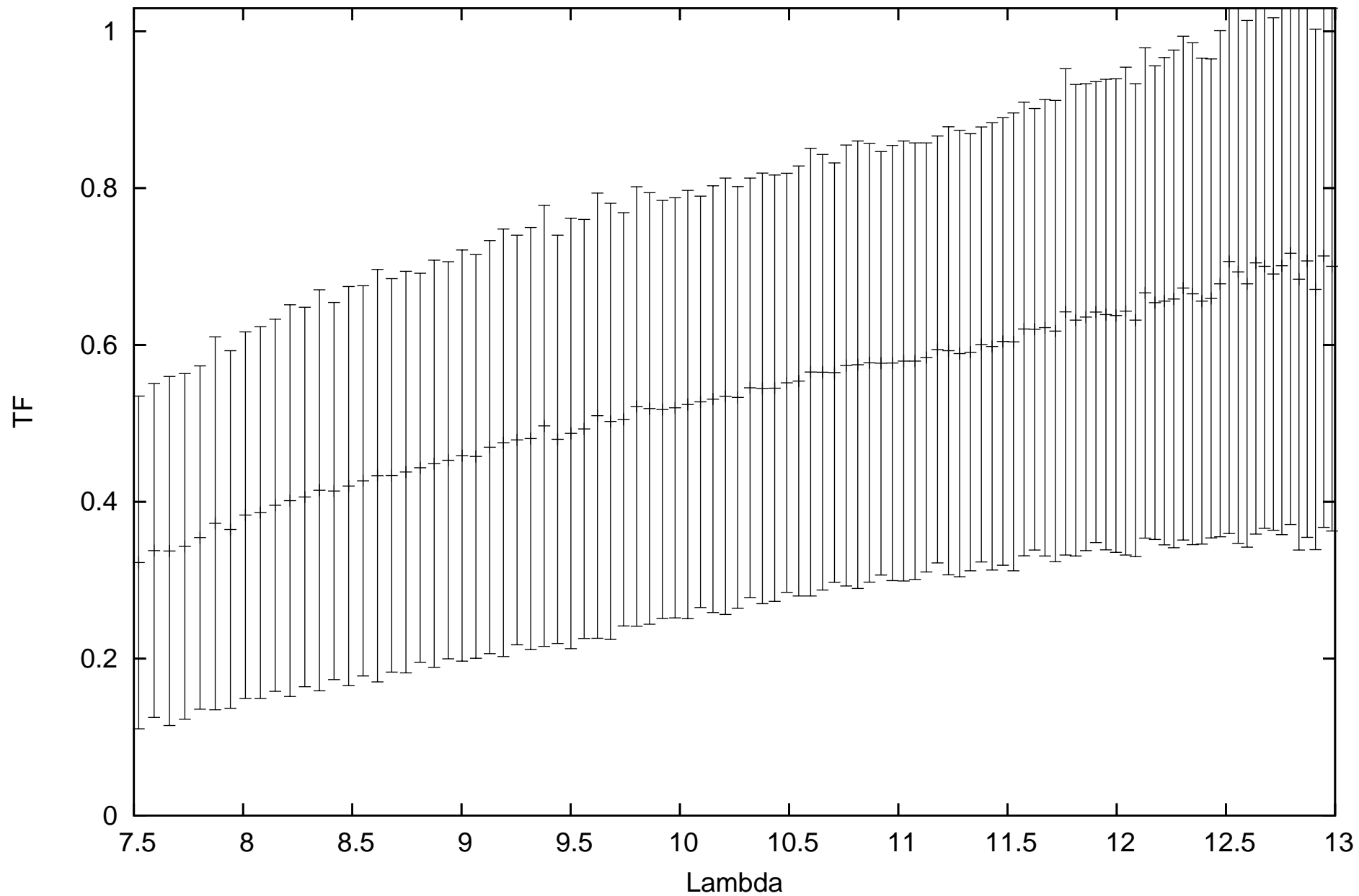
calHD167618_flux-1.82_diam11.66_r.MIDI.2009-08-17T03_04_23.000_HIGHSENS
