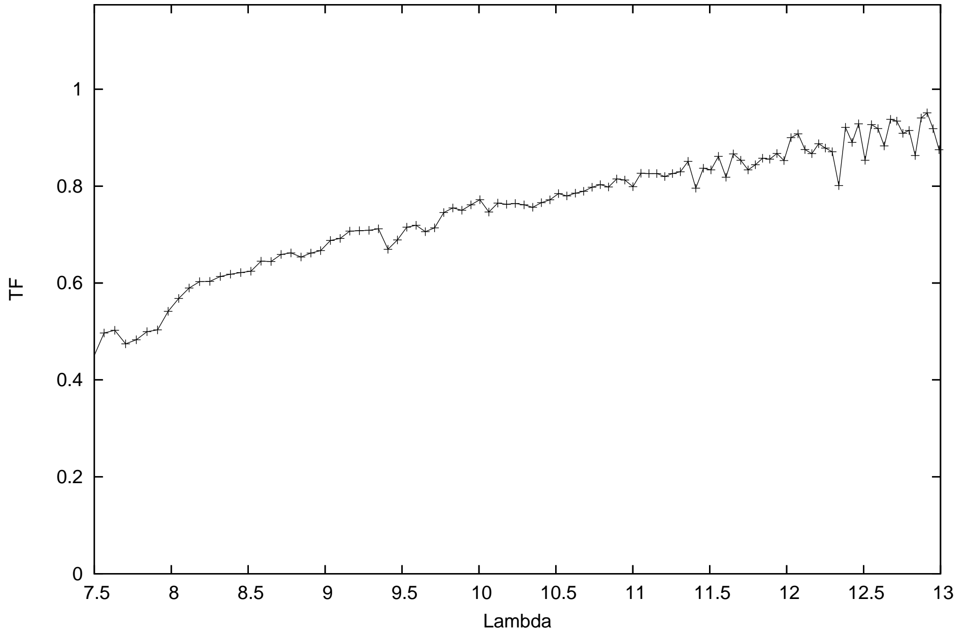
calHD167618_flux-1.82_diam11.66_r.MIDI.2009-08-14T05_17_14.645 SCIPHOT
