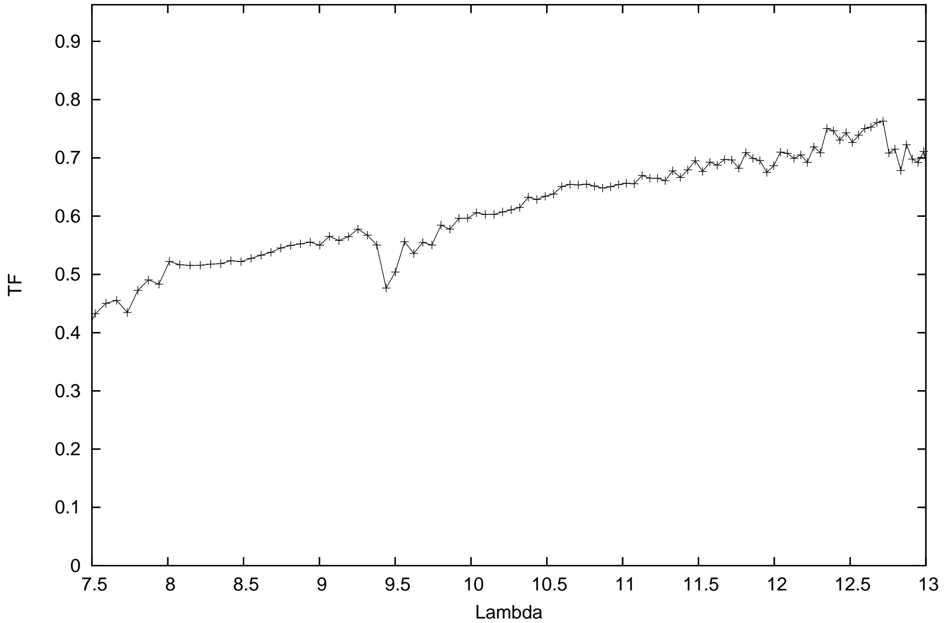
calHD167618_flux-1.82_diam11.66_r.MIDI.2009-08-11T06_22_24.000_HIGHSENS
