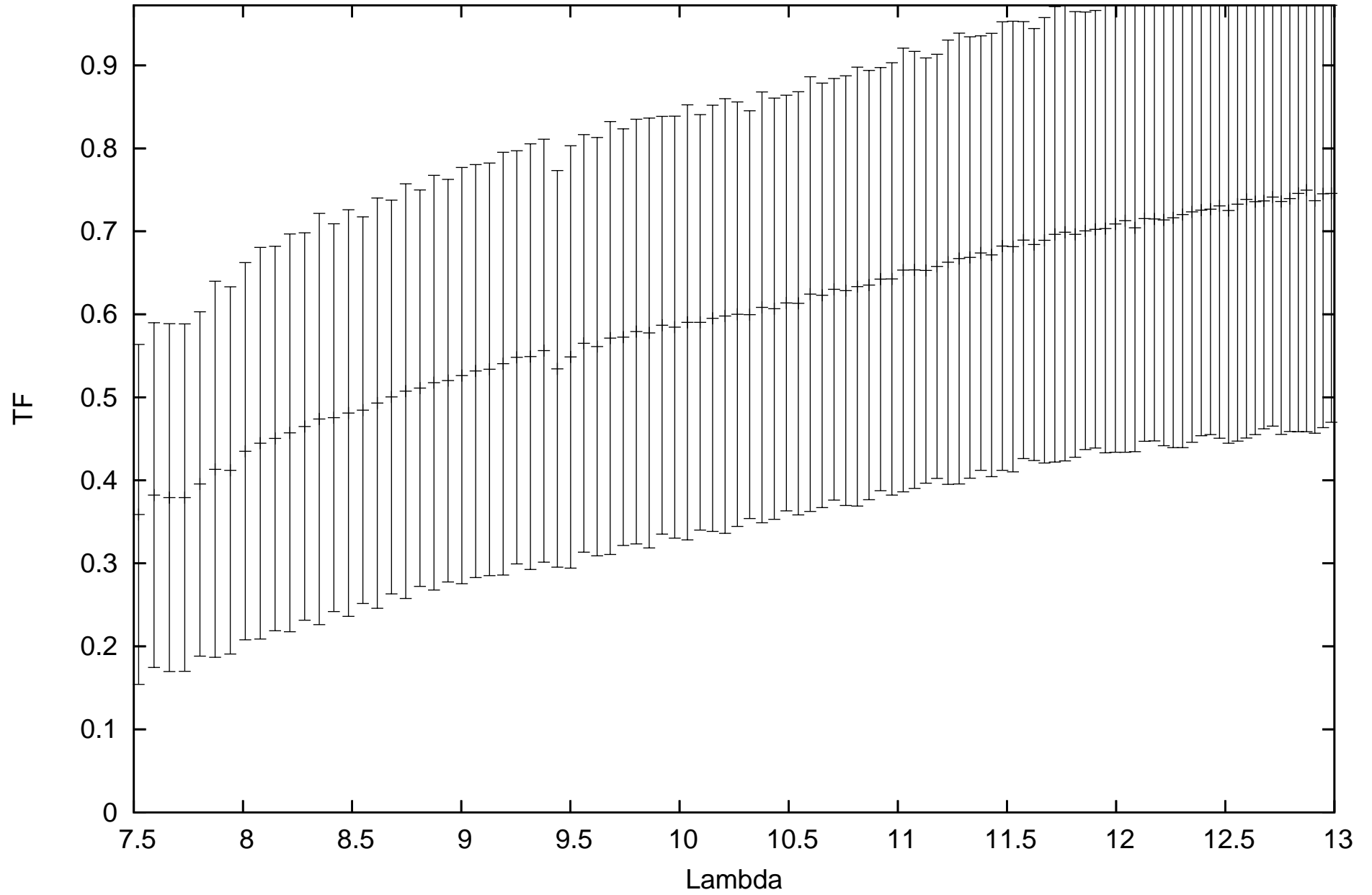
calHD167618_flux-1.82_diam11.66_r.MIDI.2009-08-02T04_11_13.000_HIGHSENS
