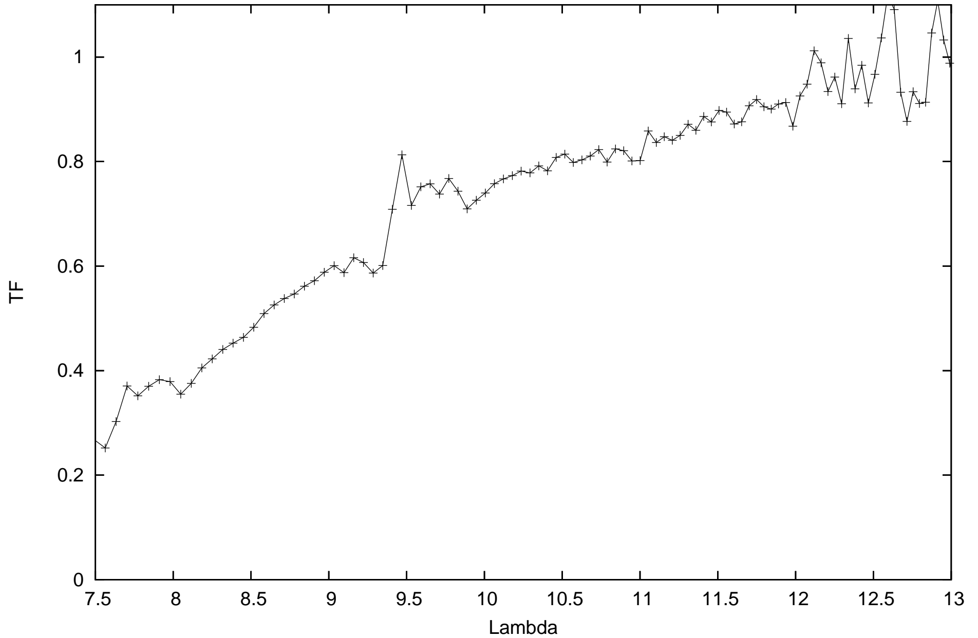
calHD167618_flux-1.82_diam11.66_r.MIDI.2009-06-03T06_37_55.686 SCIPHOT
