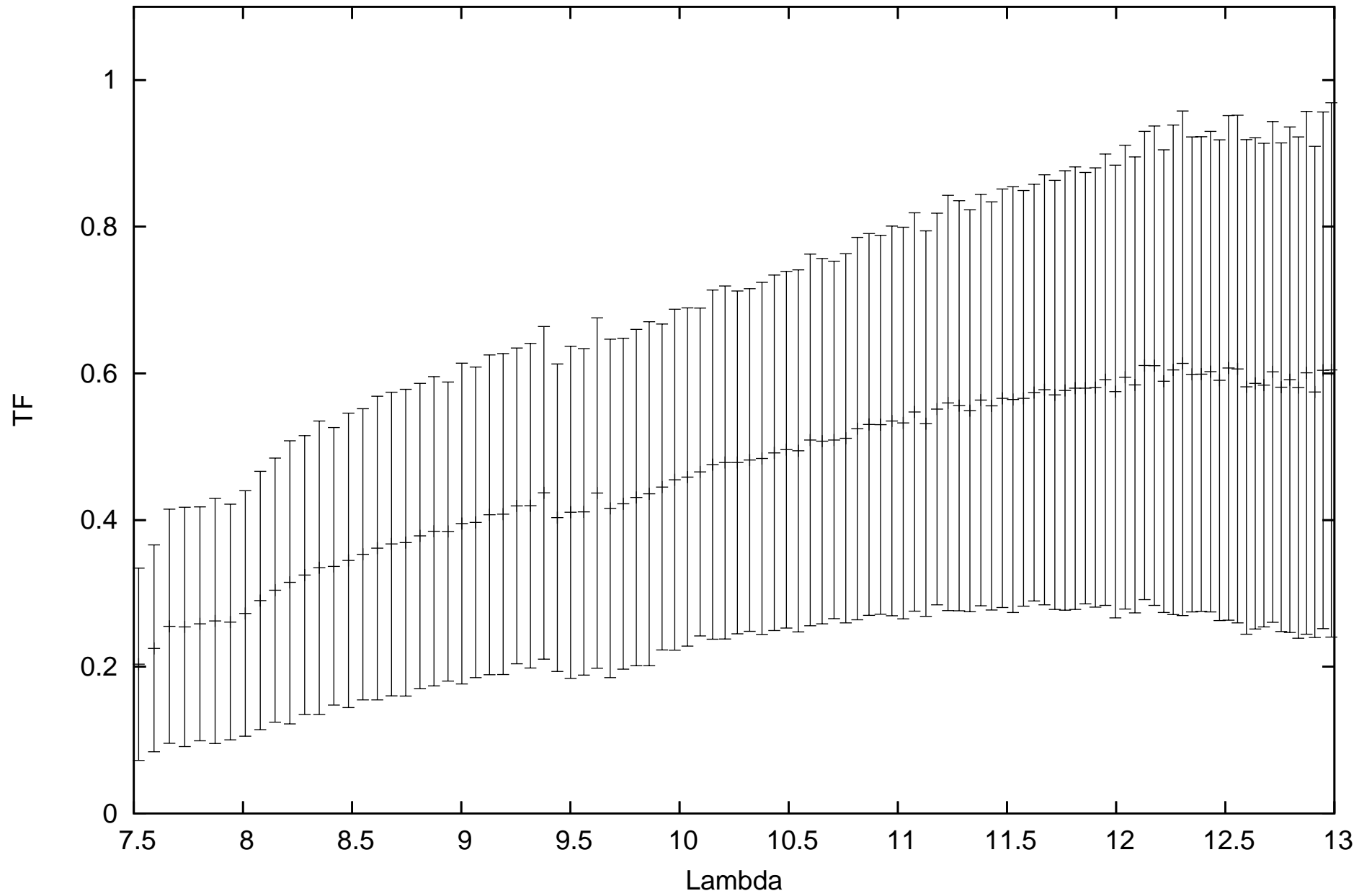
calHD167618_flux-1.82_diam11.66_r.MIDI.2008-09-27T02_14_02.000_HIGHSENS
