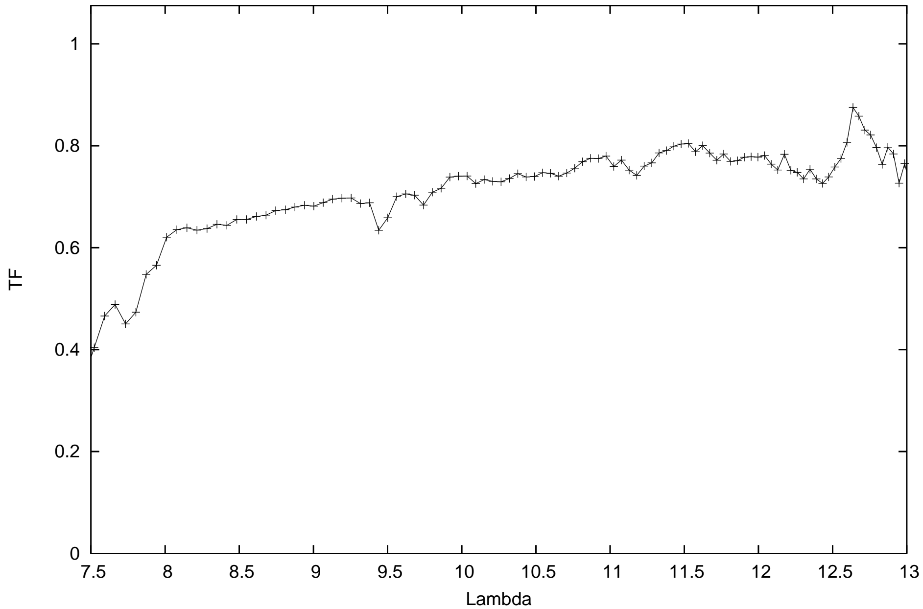
calHD156277_flux1.83_diam2._r.MIDI.2009-08-04T05_04_54.000_HIGHSENS
