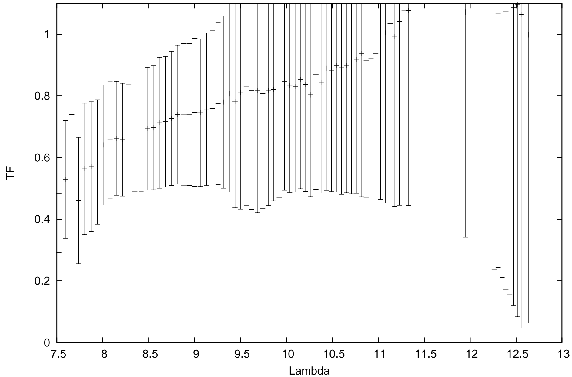
calHD152161_flux-0.26_diam6.12_r.MIDI.2009-05-04T07_51_57.000_HIGHSENS
