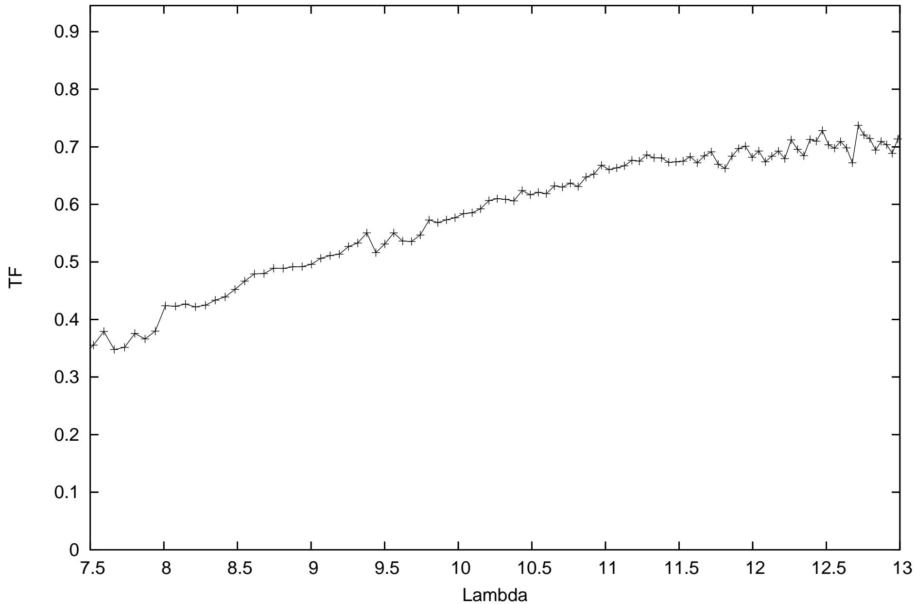
calHD127093_flux1.46_diam2.72_r.MIDI.2009-05-12T04_28_23.000_HIGHSENS
