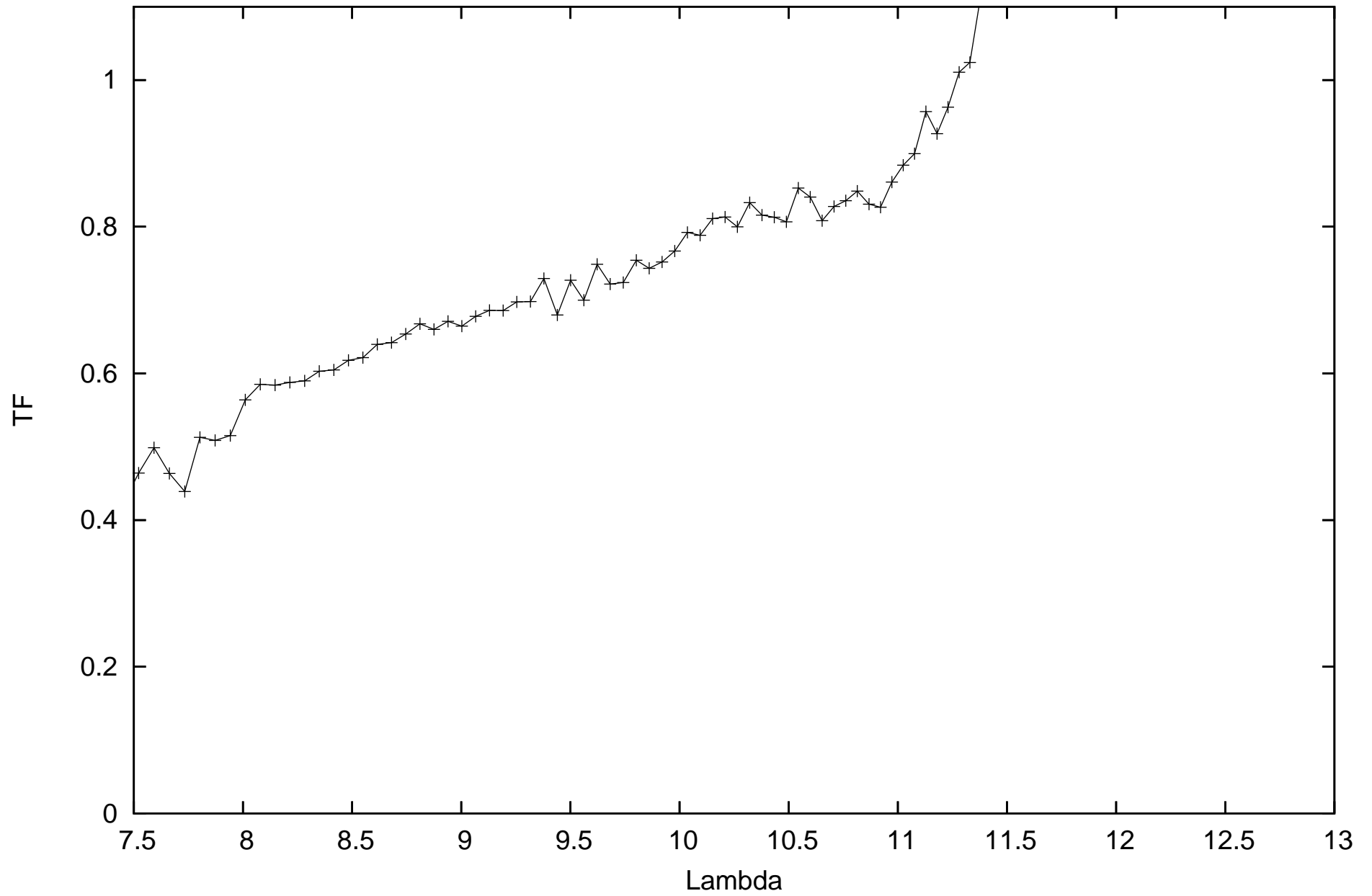
calHD123139_flux-0.39_diam5.34_r.MIDI.2009-05-04T05_33_13.000_HIGHSENS
