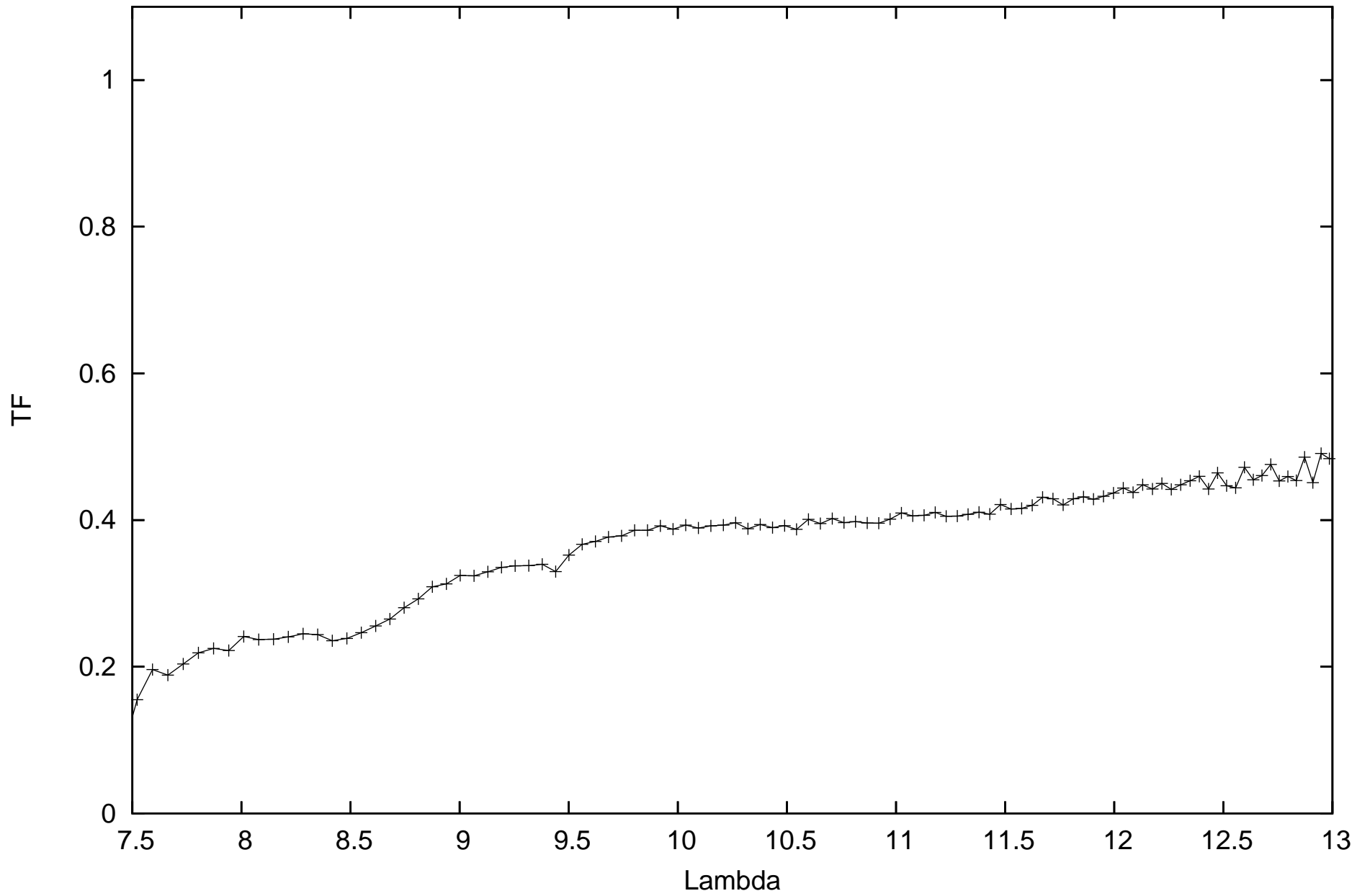
calHD120404_flux1.19_diam2.96_r.MIDI.2009-04-15T06_32_46.000_HIGHSENS
