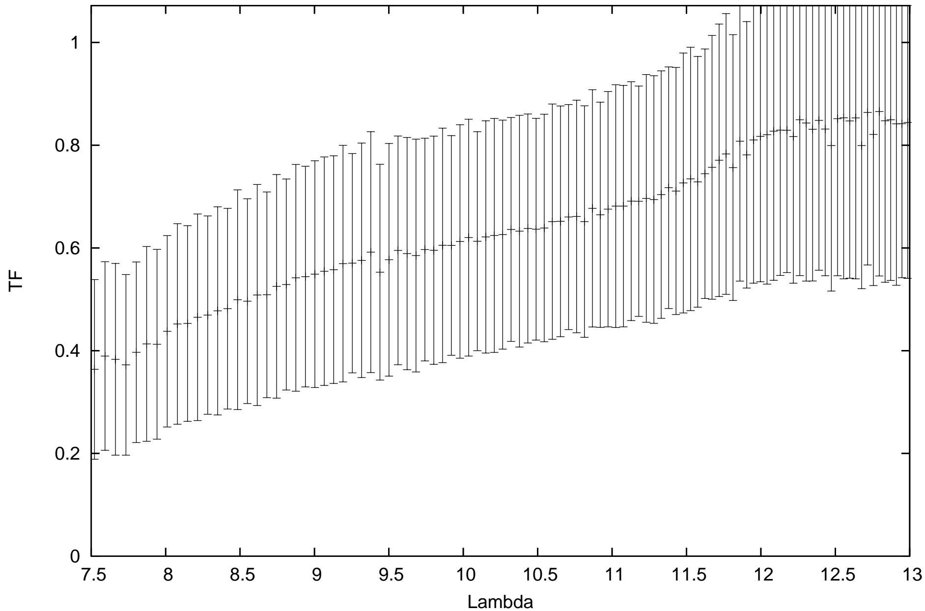
calHD120323_flux-2.02_diam13.25_r.MIDI.2009-07-06T23_45_11.000_HIGHSENS
