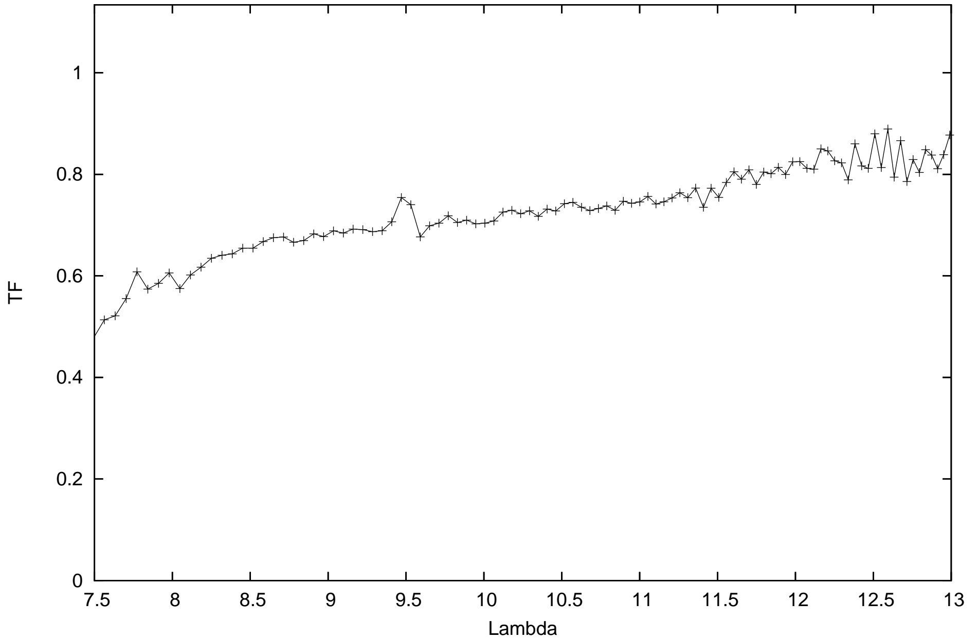
calHD120323_flux-2.02_diam13.25_r.MIDI.2009-04-24T06_21_50.945 SCIPHOT
