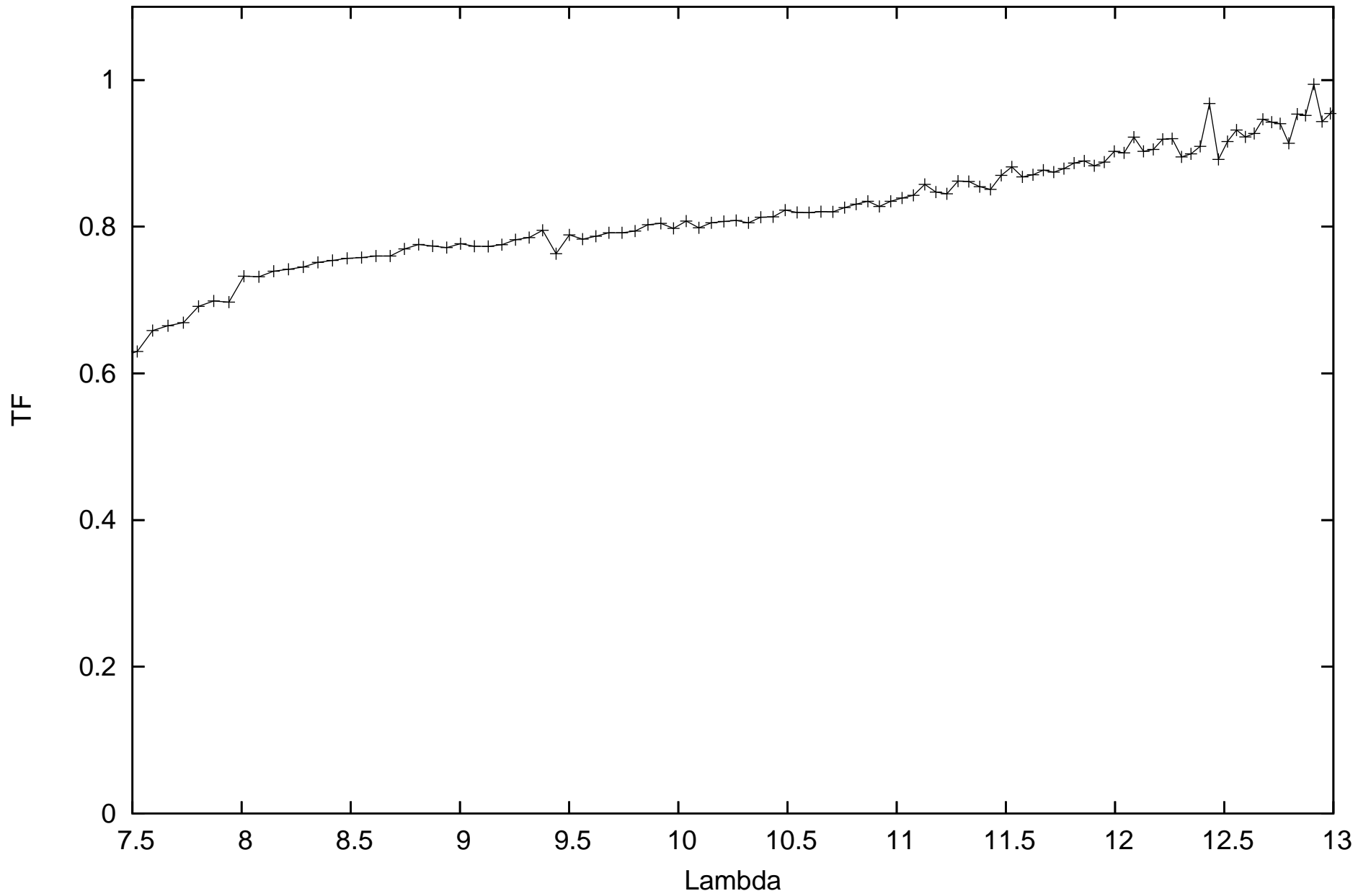
calHD120323_flux-2.02_diam13.25_r.MIDI.2009-04-24T05_25_13.000_HIGHSENS
