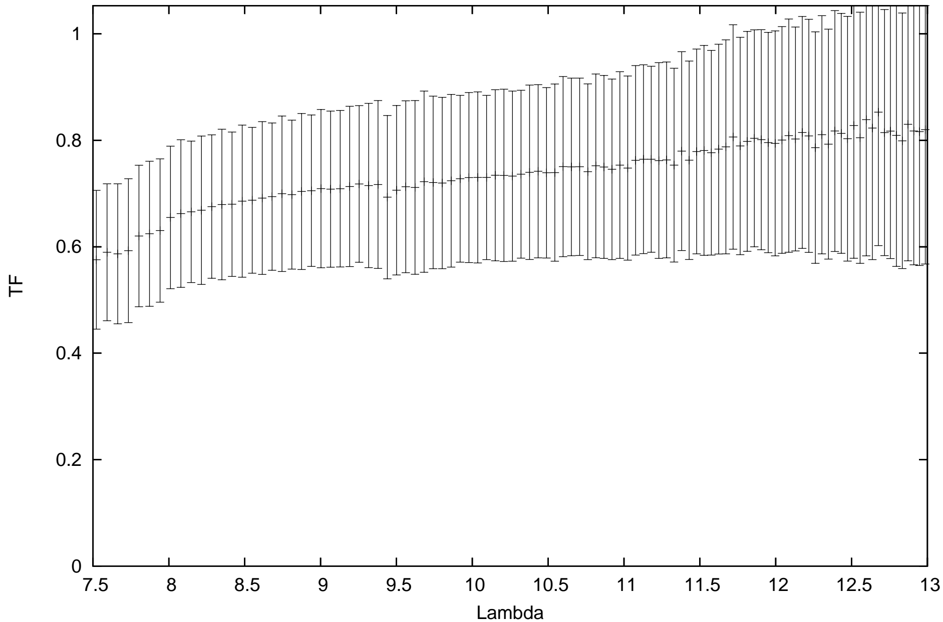
calHD120323_flux-2.02_diam13.25_r.MIDI.2009-04-24T04_44_31.000_HIGHSENS
