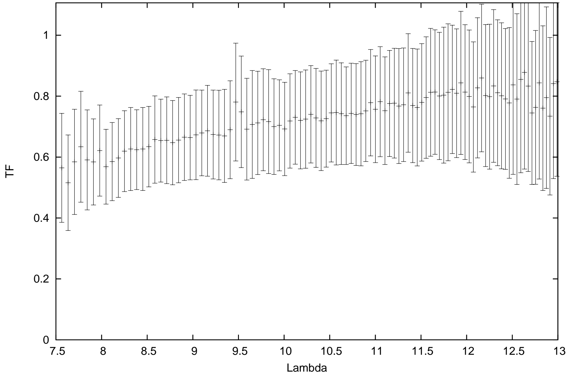
calHD120323_flux-2.02_diam13.25_r.MIDI.2009-04-23T07_38_59.110 SCIPHOT
