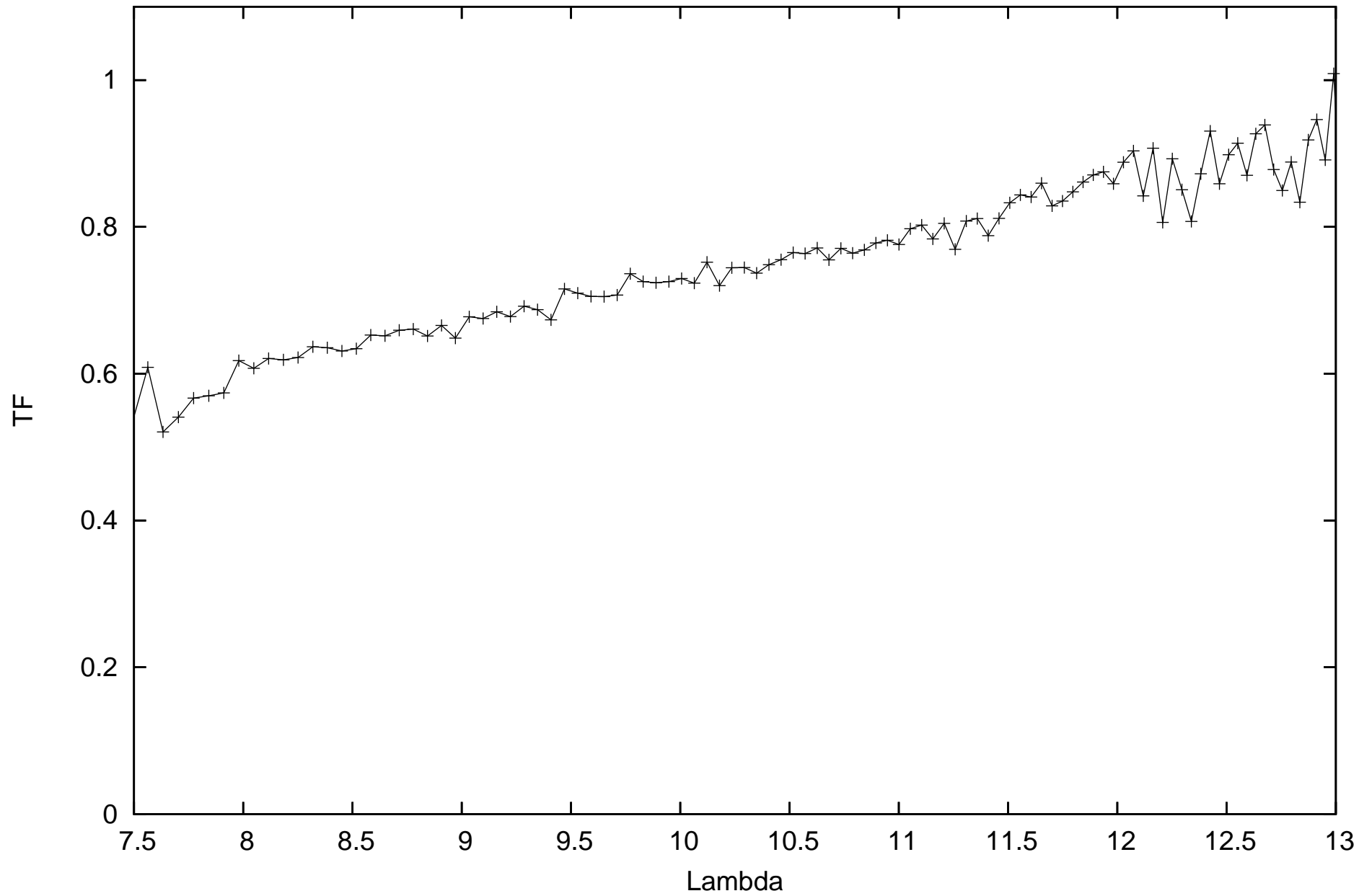
calHD120323_flux-2.02_diam13.25_r.MIDI.2009-04-20T08_36_19.110 SCIPHOT
