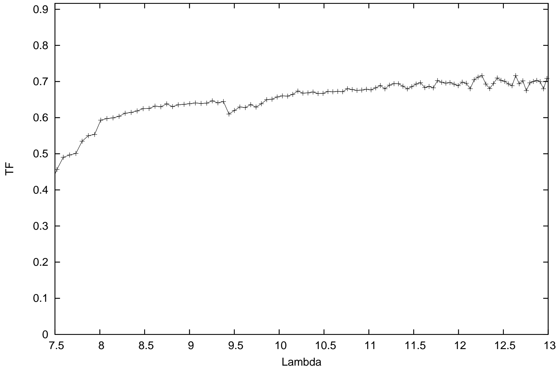
calHD112213_flux1.03_diam3.16_r.MIDI.2009-05-10T06_34_00.000_U2U4
