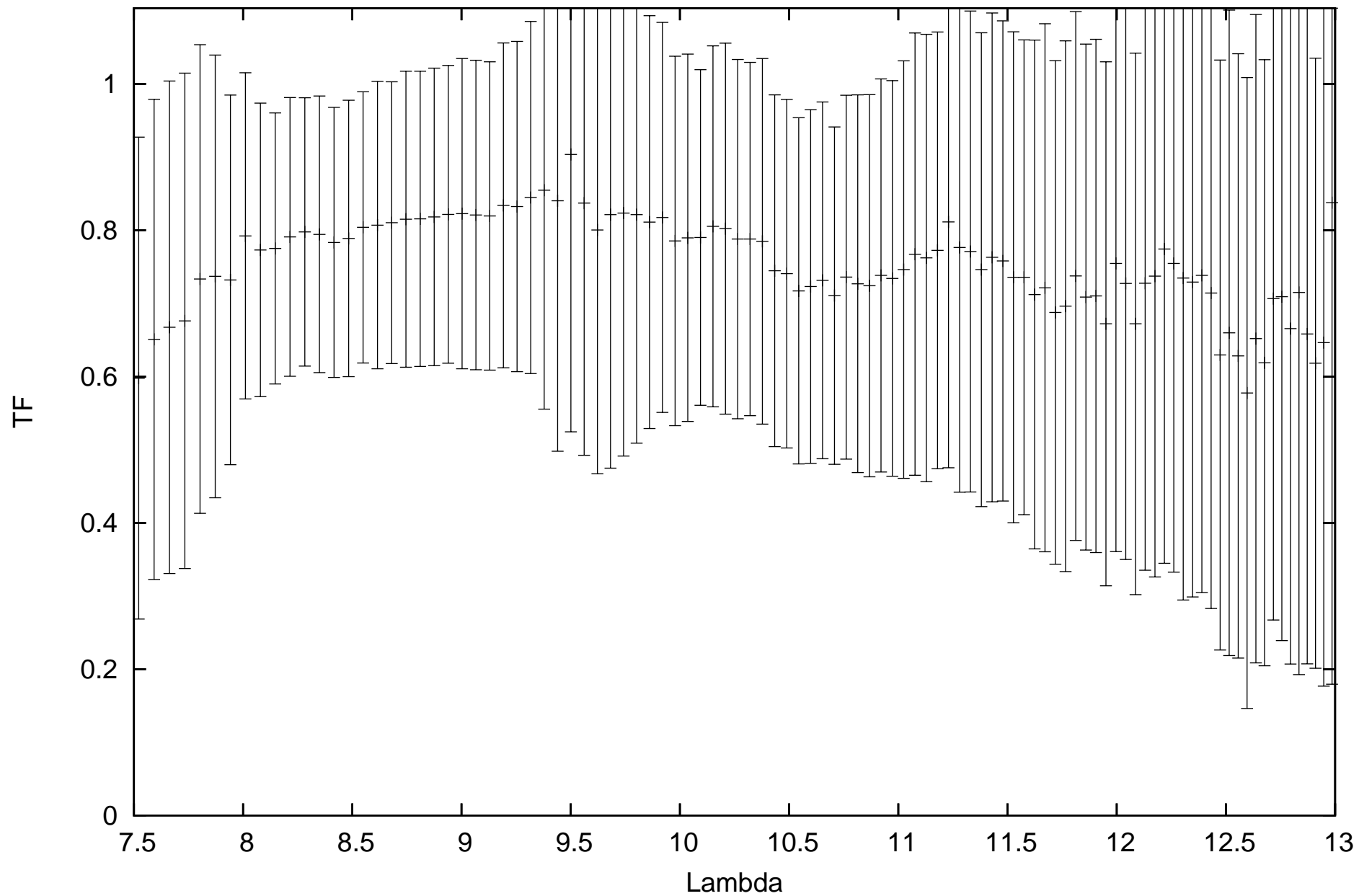
calHD107446_flux0.22_diam4.43_r.MIDI.2009-04-24T04_13_57.000_HIGHSENS
