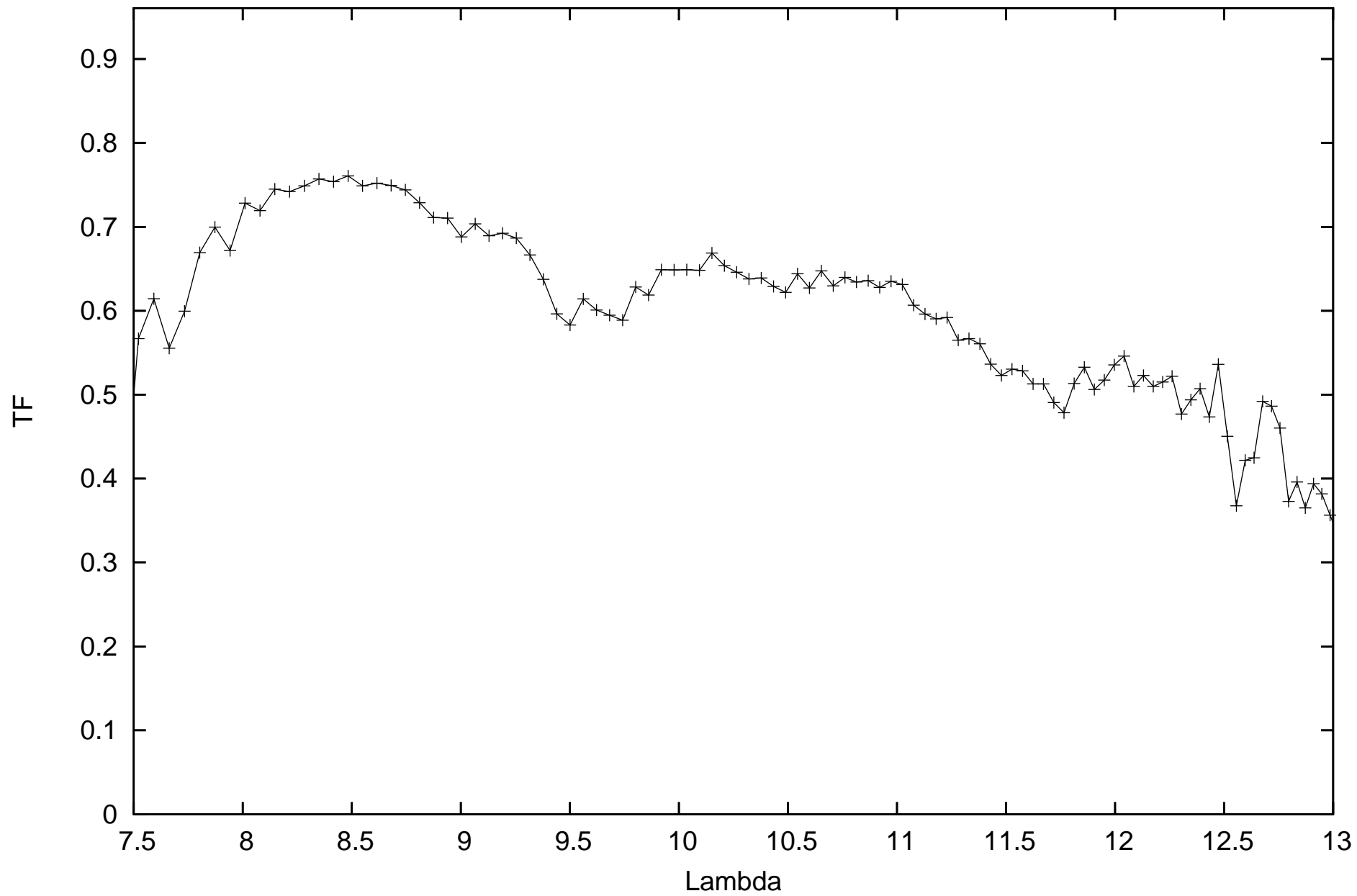
calHD107446_flux0.22_diam4.43_r.MIDI.2009-04-24T03_43_45.000_HIGHSENS
