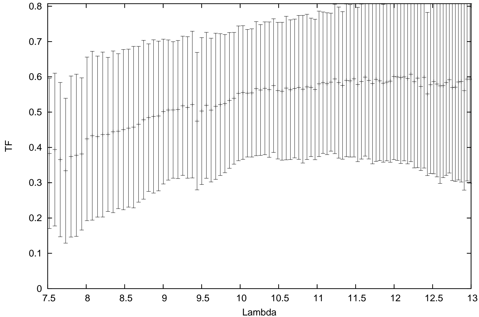
calHD094264_flux1.25_diam2.6_r.MIDI.2009-05-12T01_38_58.000_HIGHSENS
