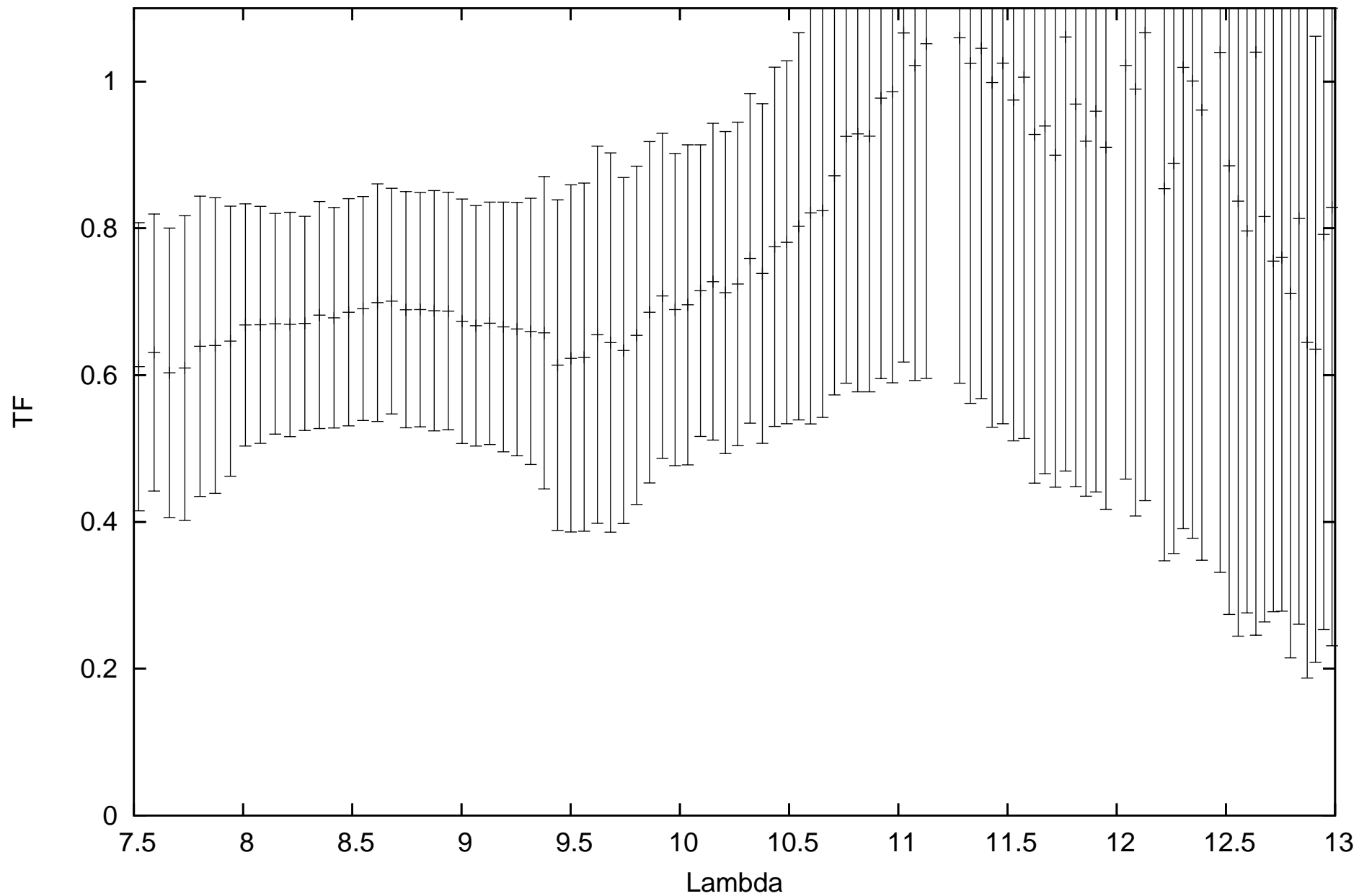
calHD093813_flux0.14_diam4.43_r.MIDI.2009-04-21T01_59_32.000_HIGHSENS
