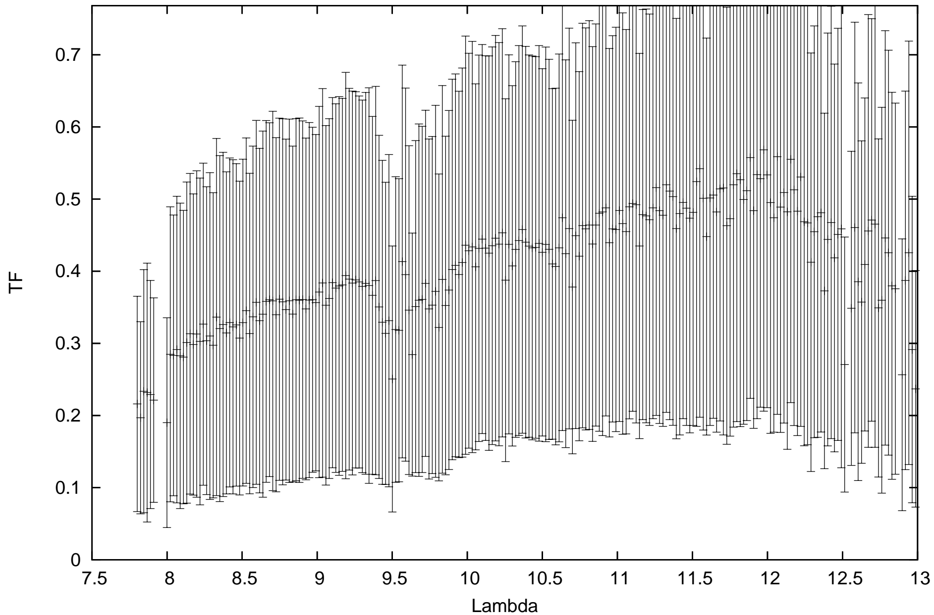
calHD089388_flux-0.2_diam5.18_r.MIDI.2010-01-17T08_20_56.000_E0G0
