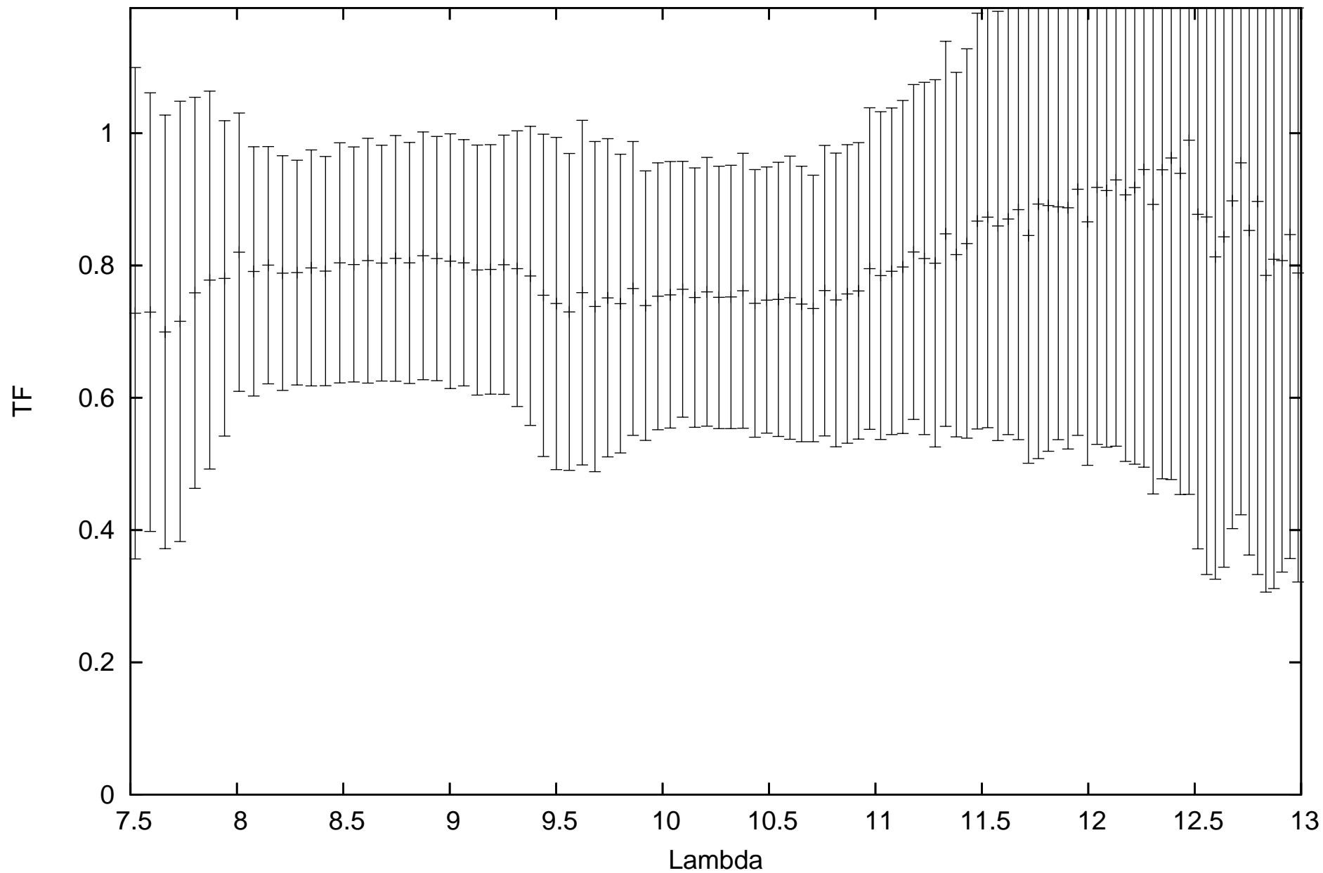
calHD089388_flux-0.2_diam5.18_r.MIDI.2009-04-24T02_16_35.000_HIGHSENS
