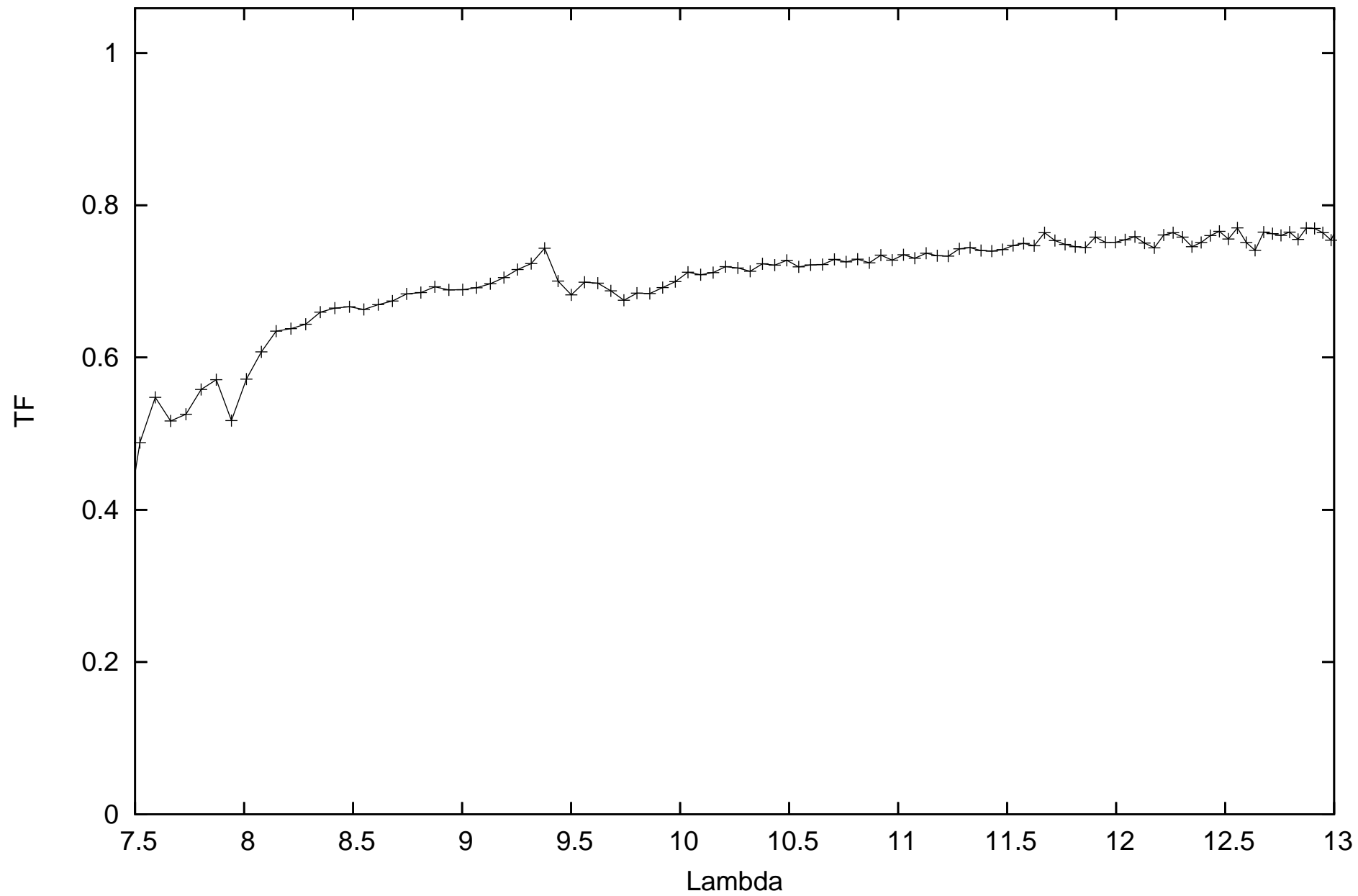
calHD083618_flux0.76_diam3.36_r.MIDI.2010-02-01T06_10_48.000_U3U4
