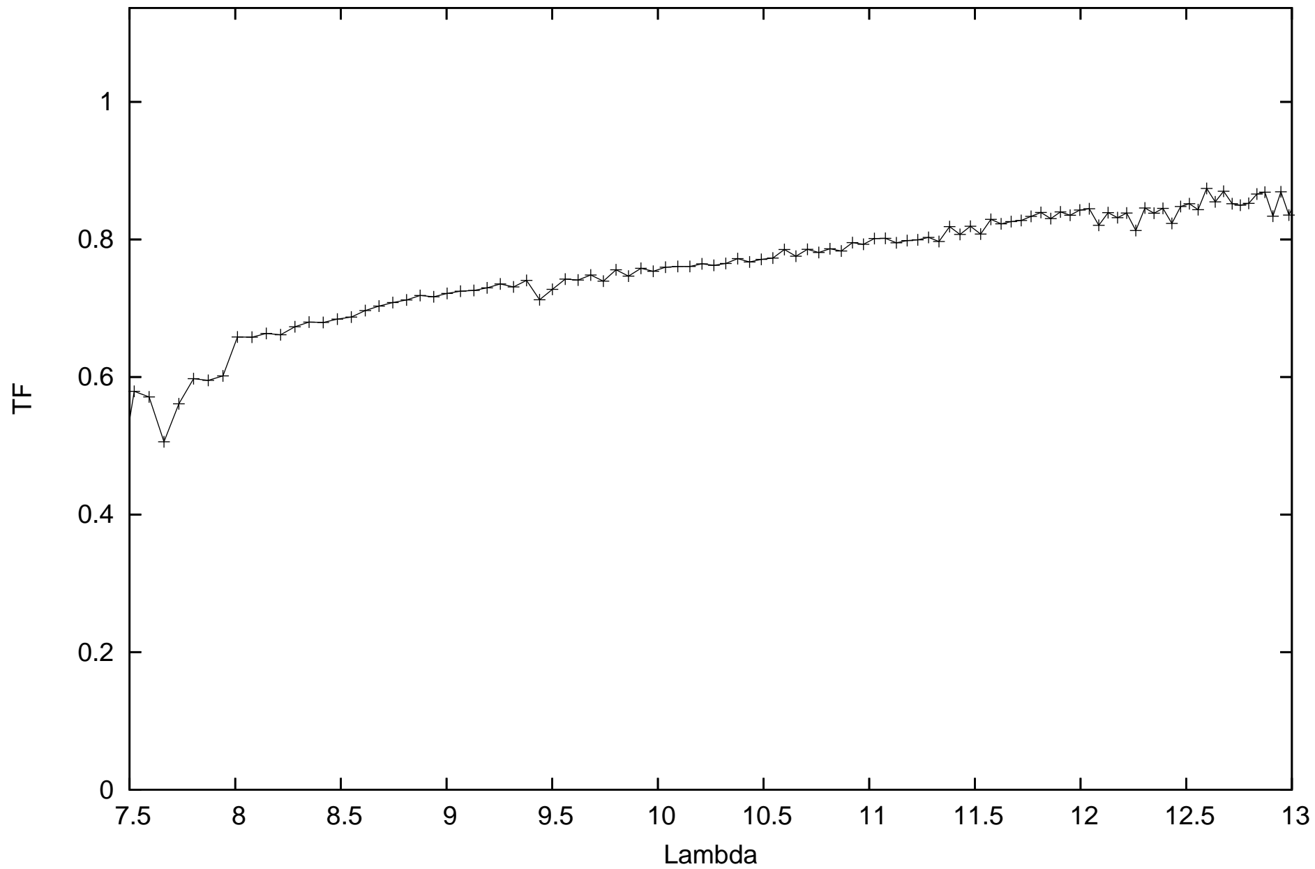
calHD083618_flux0.76_diam3.36_r.MIDI.2010-01-31T06_53_16.000_U2U4
