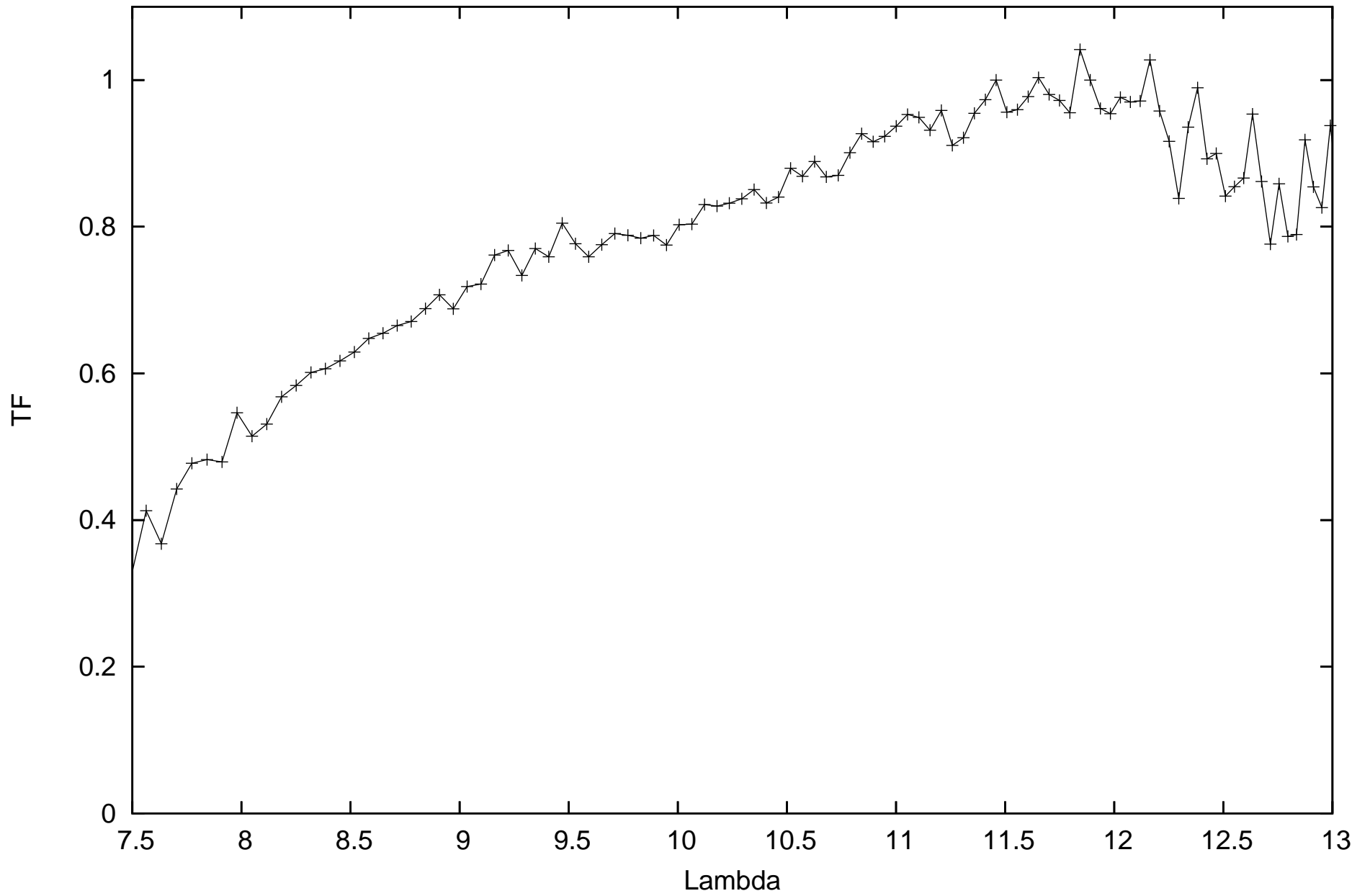
calHD081797_flux-1.49_diam9.14_r.MIDI.2010-02-05T06_57_43.522_H0D0
