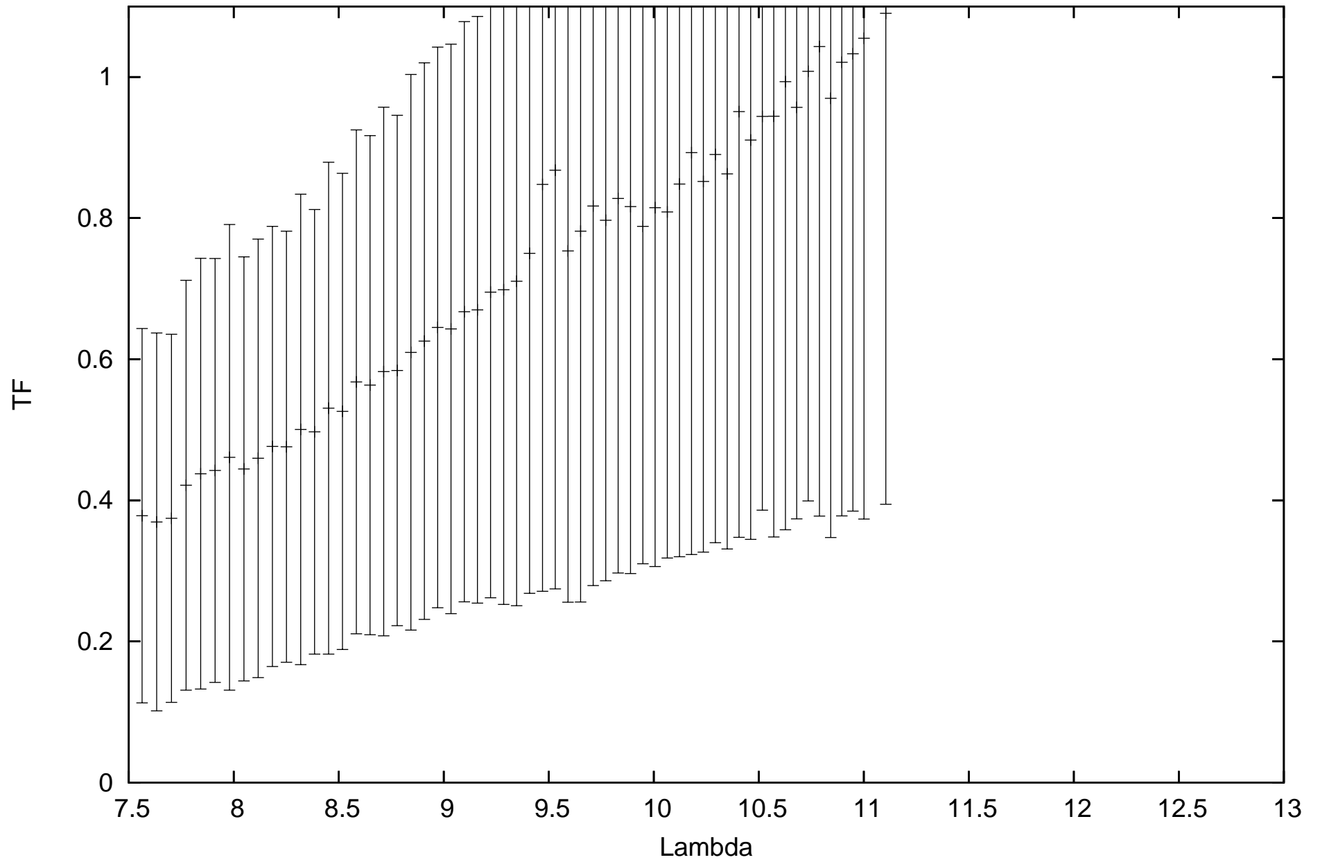
calHD081797_flux-1.49_diam9.14_r.MIDI.2010-02-04T07_24_04.316_G1D0
