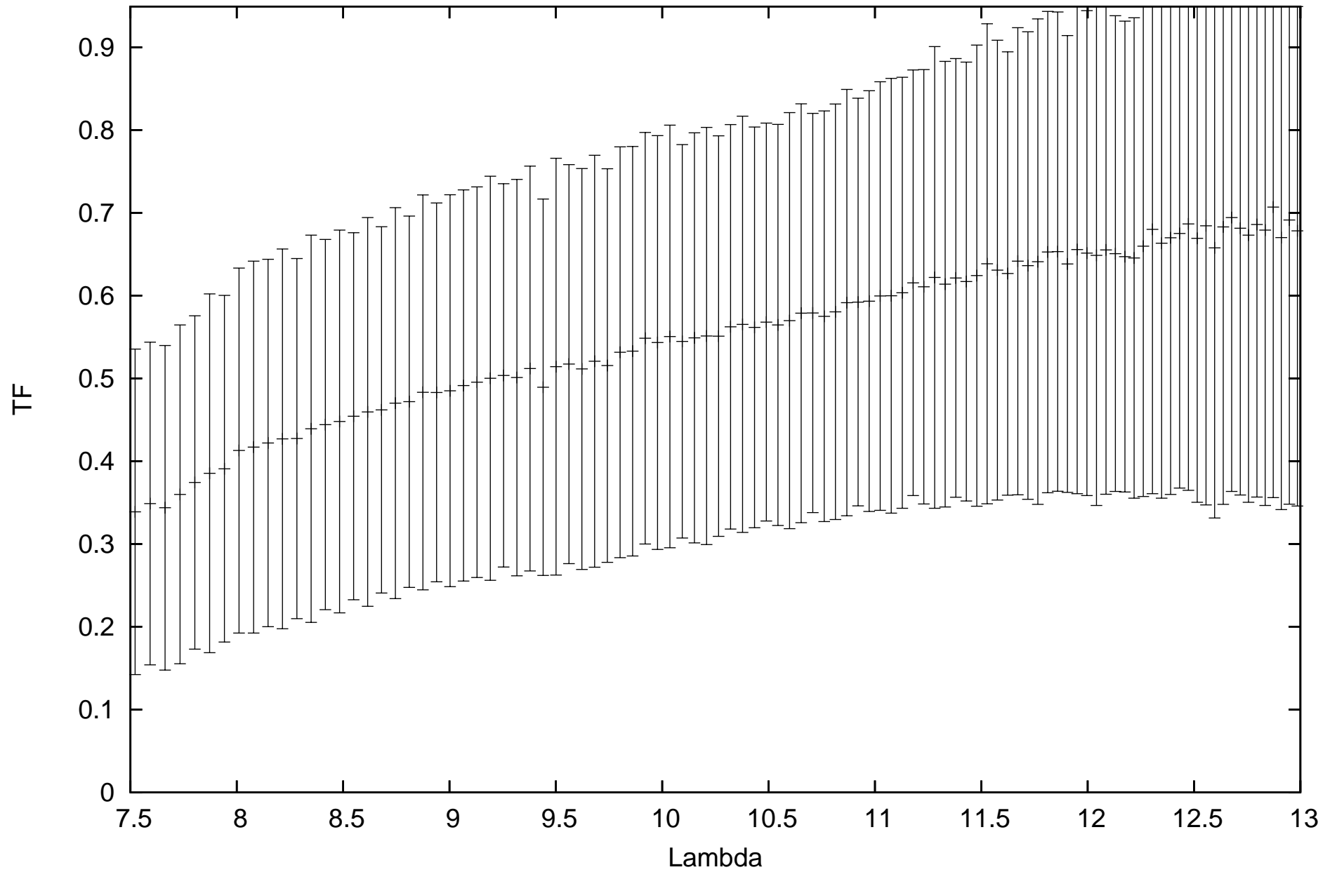
calHD081797_flux-1.49_diam9.14_r.MIDI.2010-02-04T07_15_12.000_G1D0
