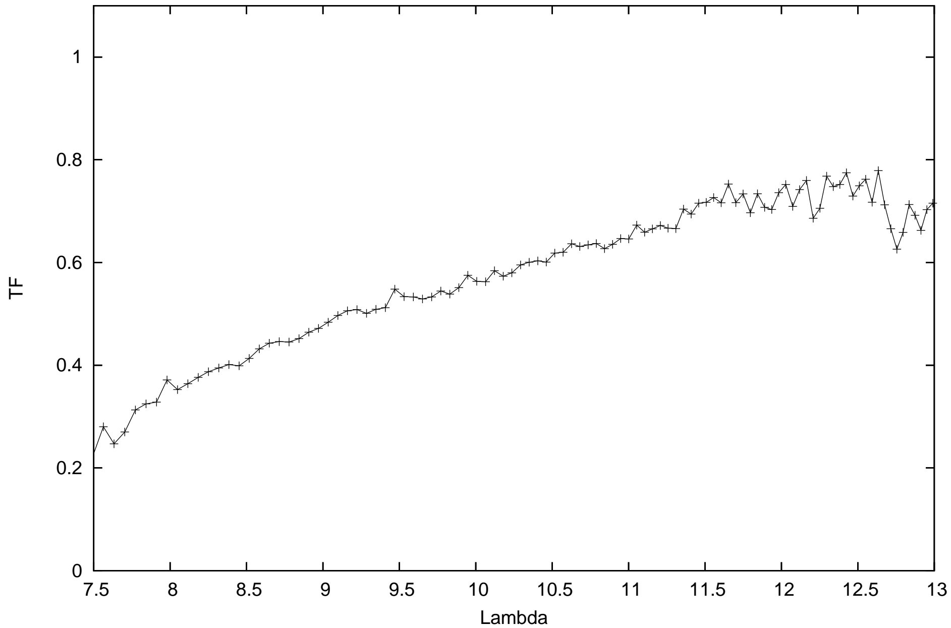
calHD081797_flux-1.49_diam9.14_r.MIDI.2010-01-26T08_43_45.987_K0G1
