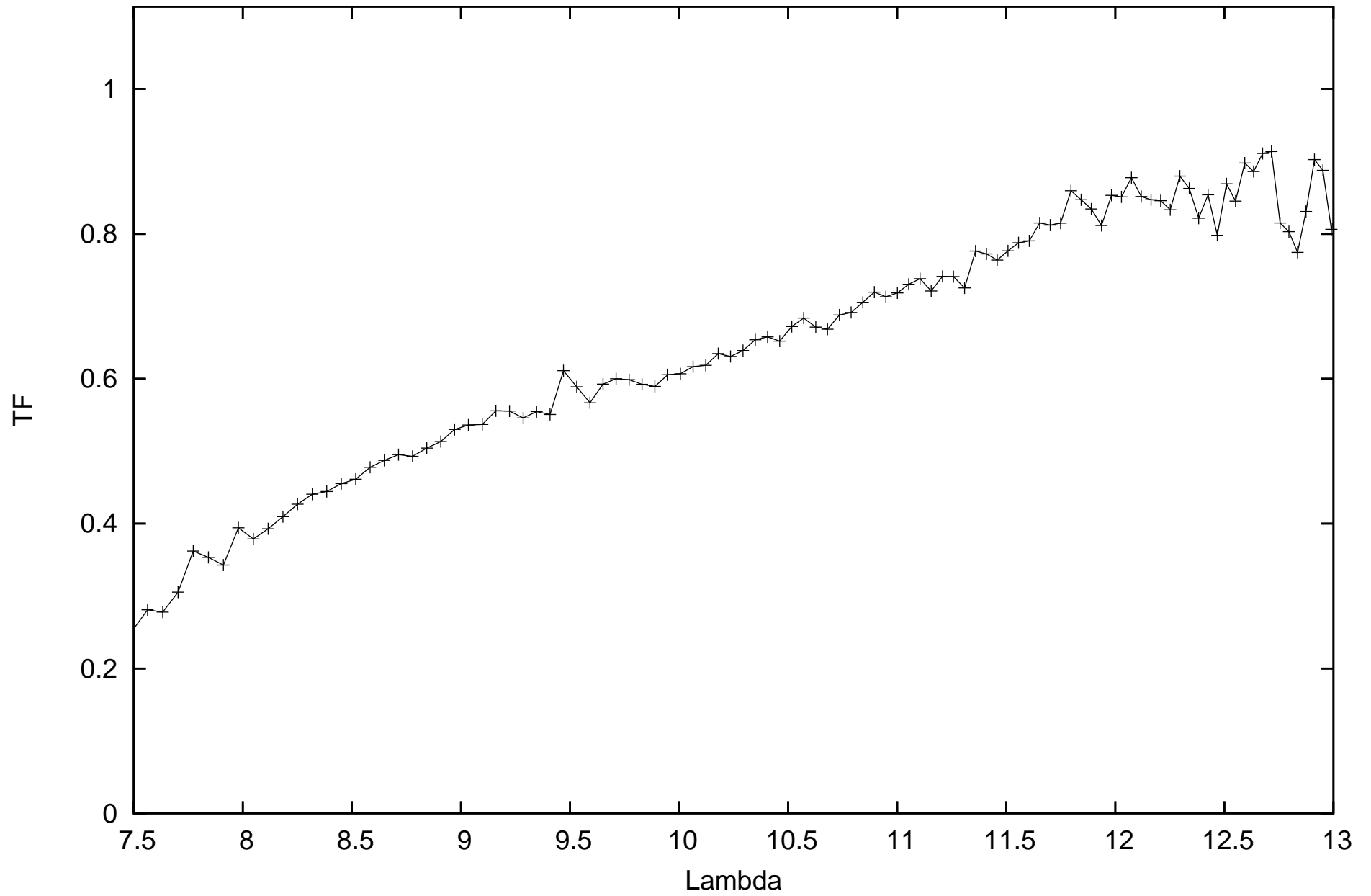
calHD081797_flux-1.49_diam9.14_r.MIDI.2010-01-25T08_10_33.480_K0A0
