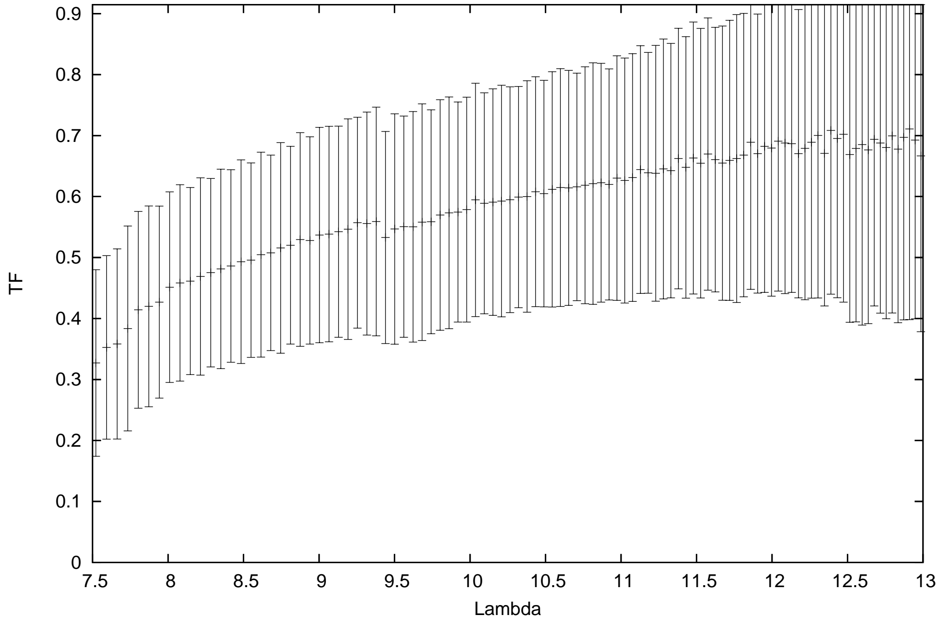
calHD081797_flux-1.49_diam9.14_r.MIDI.2010-01-25T08_01_41.000_K0A0
