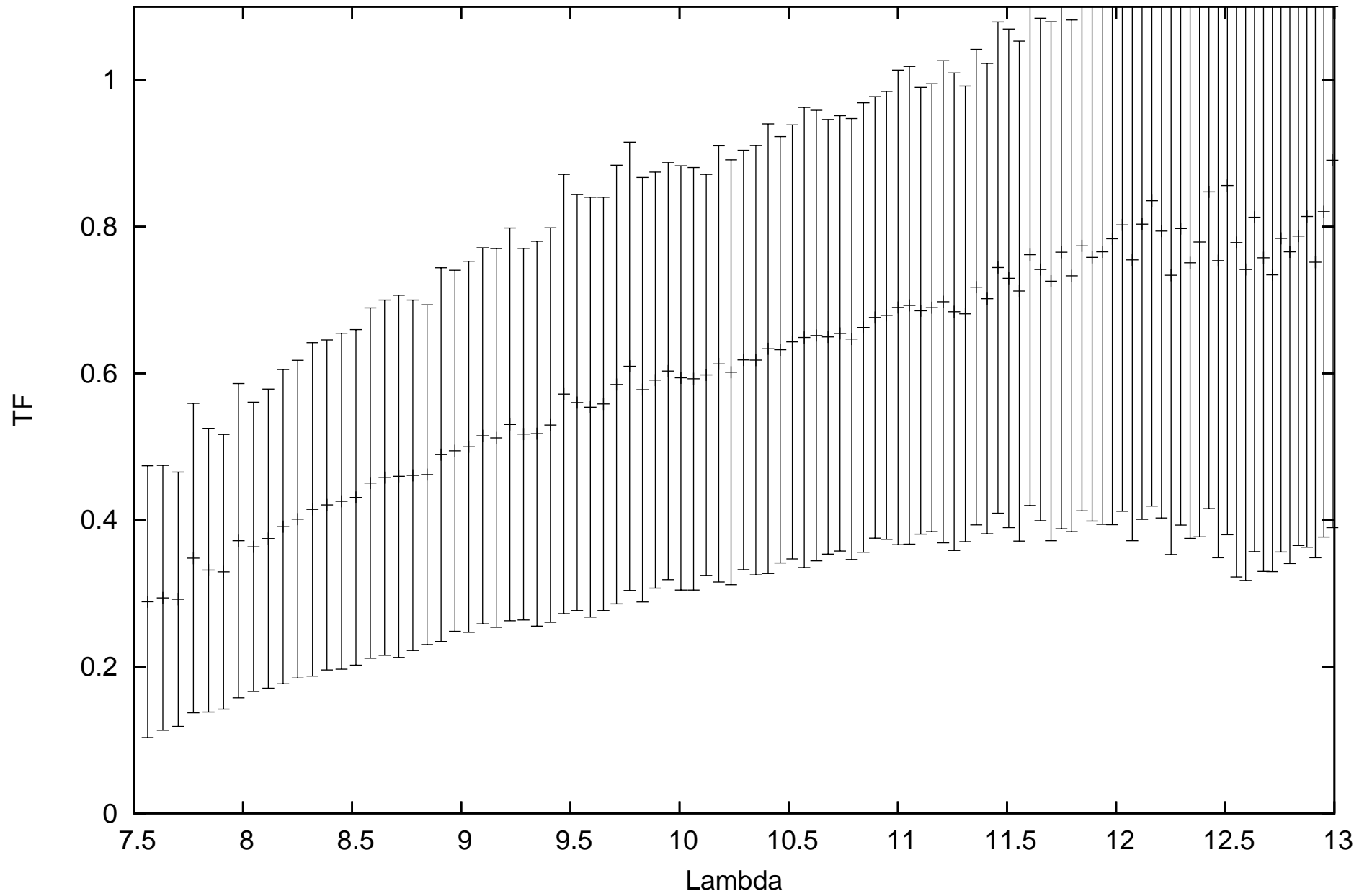
calHD081797_flux-1.49_diam9.14_r.MIDI.2010-01-19T06_26_29.687_G1H0
