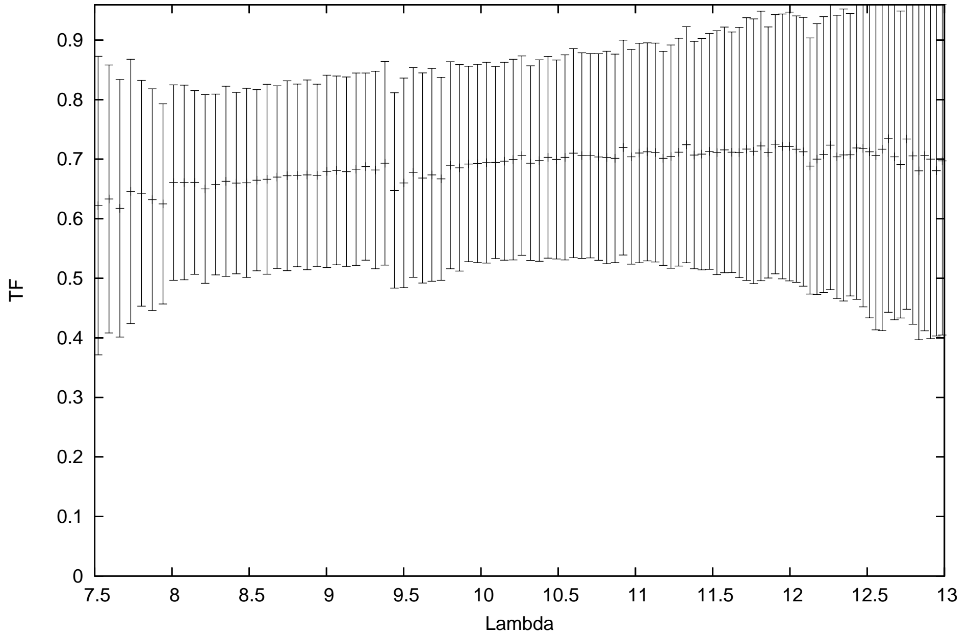
calHD081797_flux-1.49_diam9.14_r.MIDI.2010-01-13T08_31_20.000_H0D0
