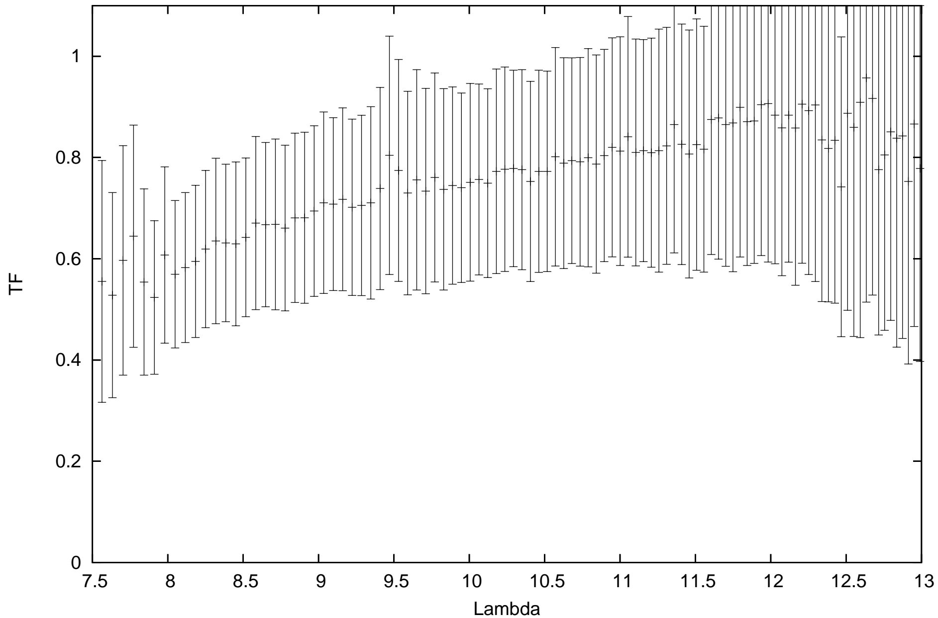
calHD081797_flux-1.49_diam9.14_r.MIDI.2010-01-13T06_49_29.357_H0D0
