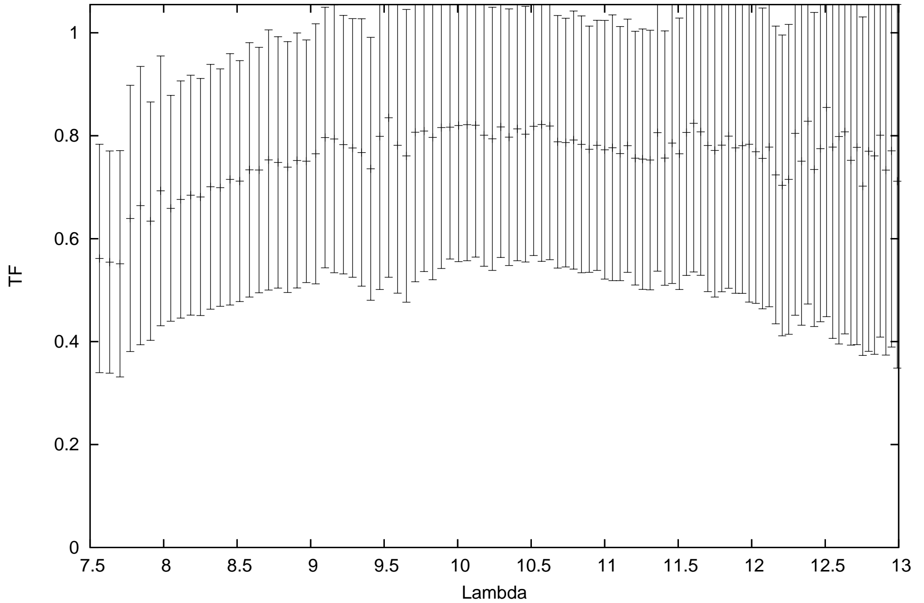
calHD081797_flux-1.49_diam9.14_r.MIDI.2009-07-05T23_00_36.316 SCIPHOT
