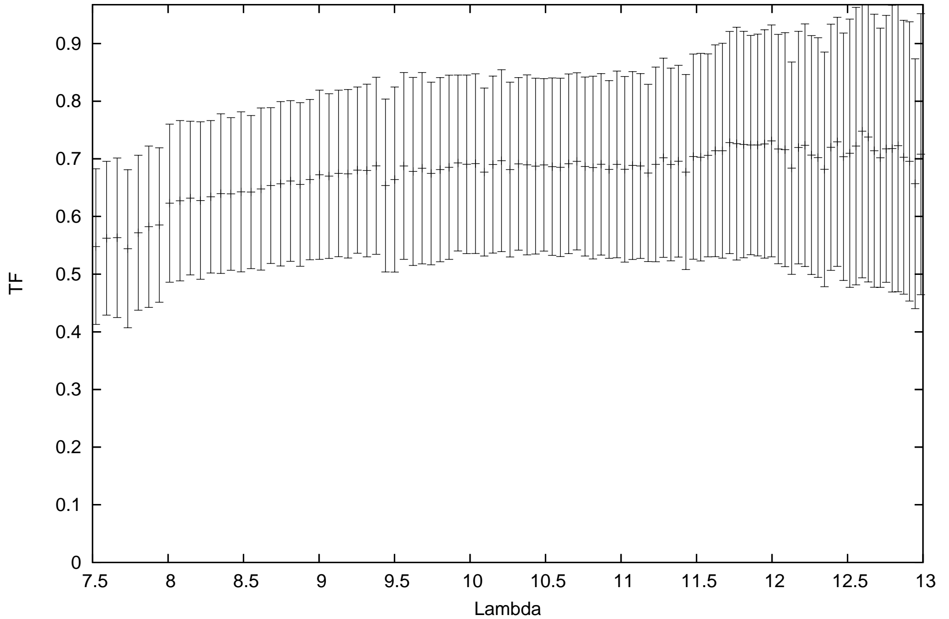
calHD081797_flux-1.49_diam9.14_r.MIDI.2009-05-02T00_22_06.000_HIGHSENS
