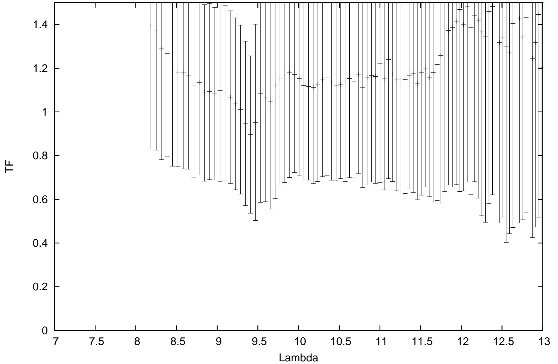
calHD081797_flux-1.49_diam9.14_r.MIDI.2009-01-22T06_27_45.015 SCIPHOT
