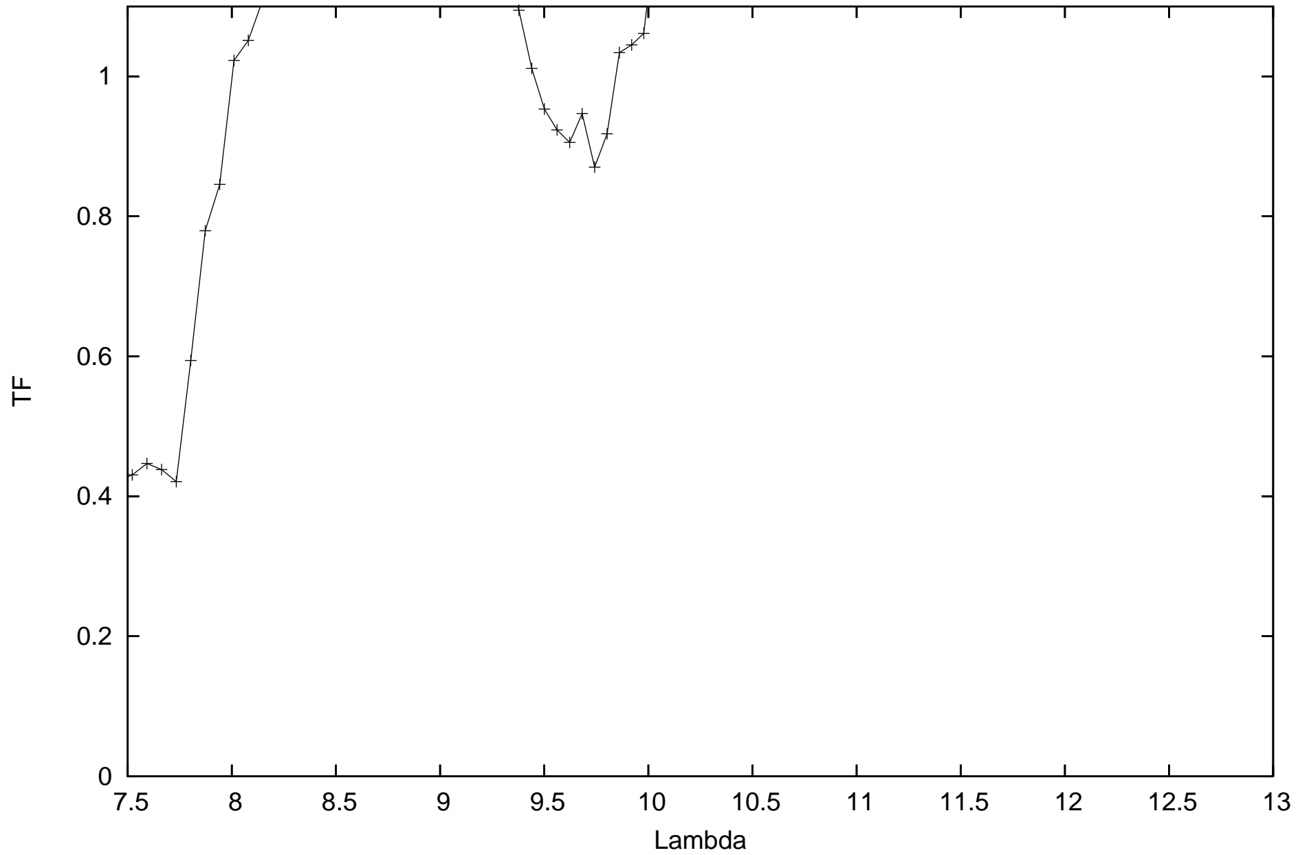
calHD081420_flux1.83_diam3.18_r.MIDI.2010-01-30T08_46_52.000_U2U4
