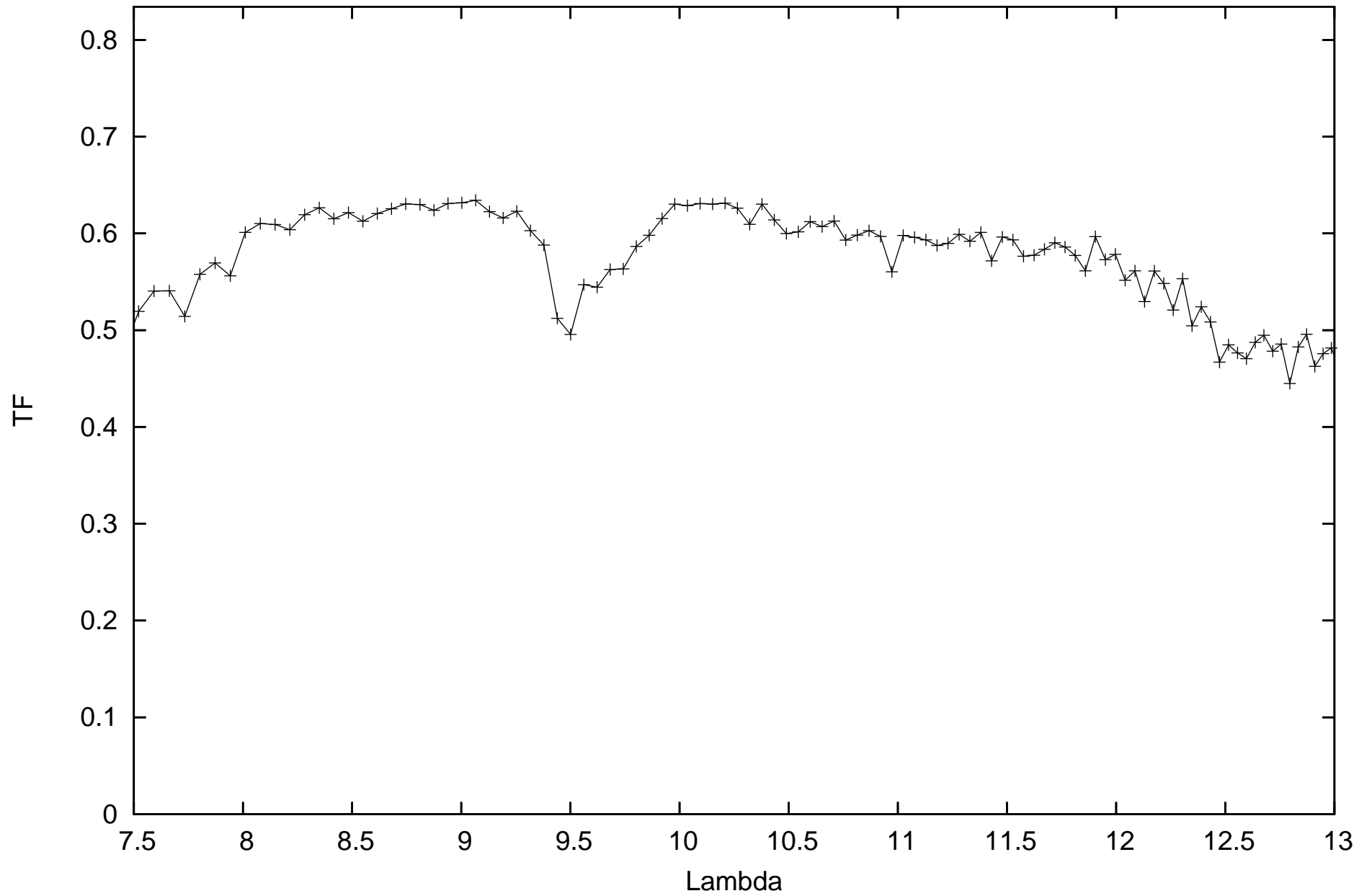
calHD065183_flux-0.08_diam5.41_r.MIDI.2010-01-04T08_26_07.000_K0G1
