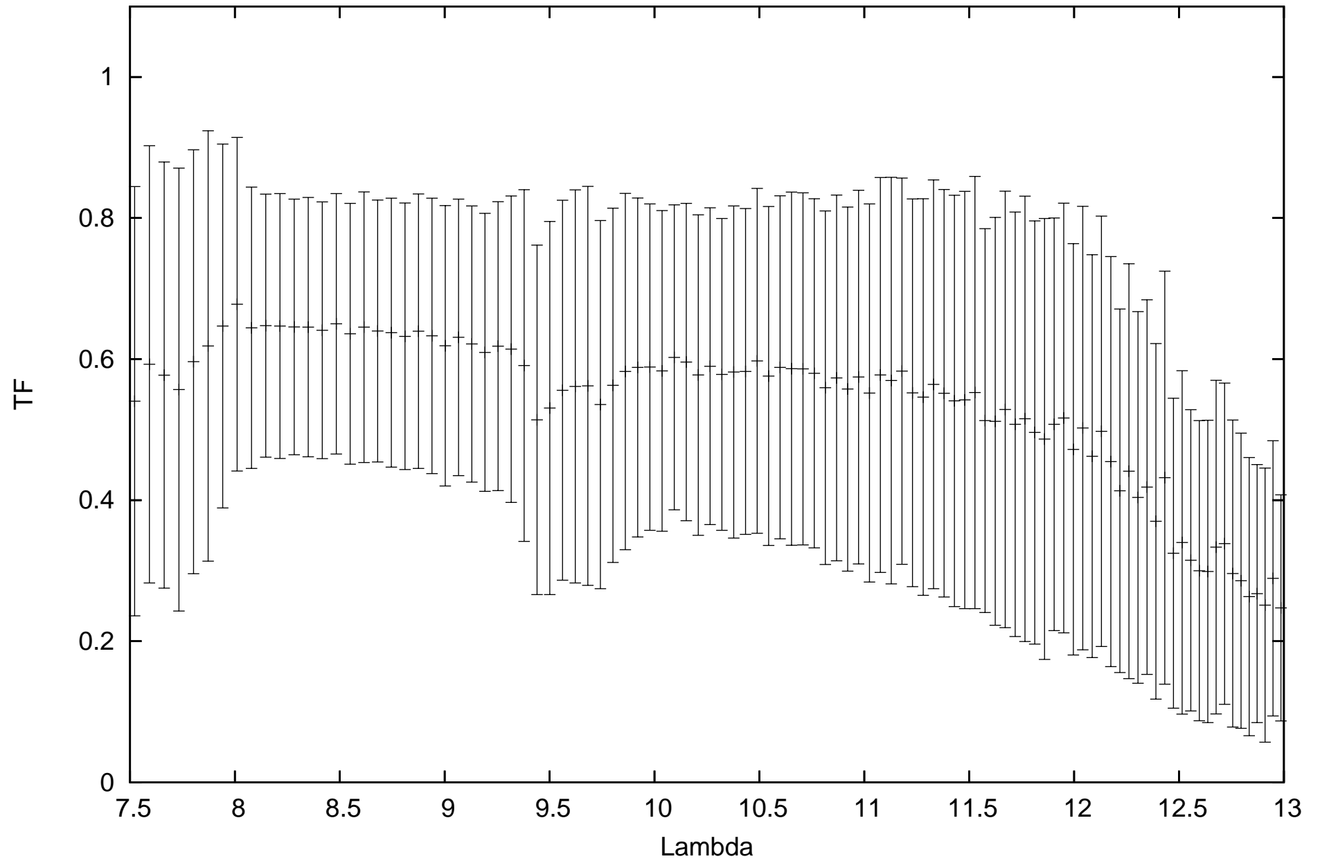
calHD062576_flux0.59_diam3.92_r.MIDI.2009-12-27T07_04_54.000_K0A0
