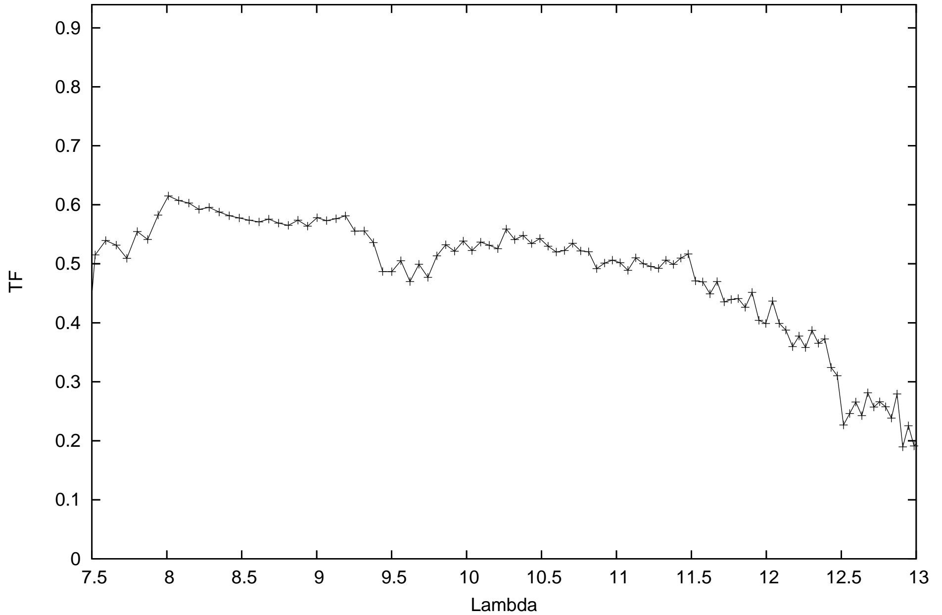
calHD062576_flux0.59_diam3.92_r.MIDI.2009-12-27T06_39_26.000_K0A0
