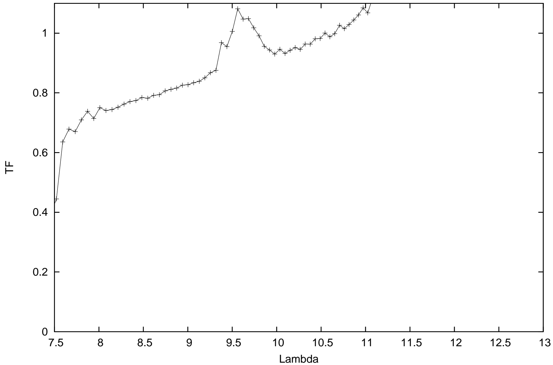
calHD061935_flux1.48_diam2.24_r.MIDI.2010-01-30T07_28_43.000_U2U4
